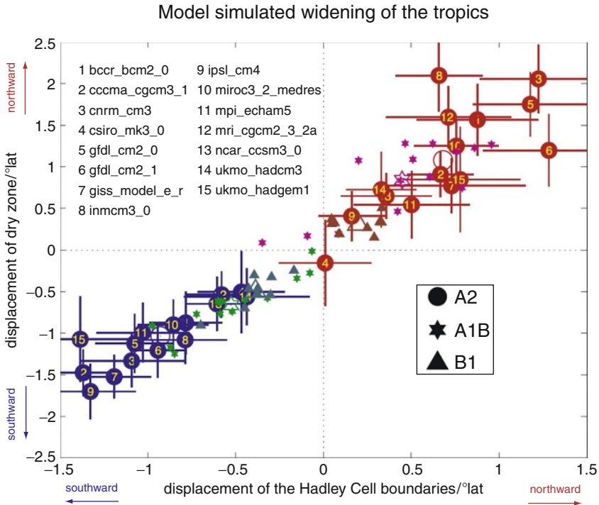
FIGURE 4 Displacements of (x-axis) the poleward boundaries of the tropical HC and (y-axis) the subtropical dry zone for different GCMs and scenarios. Reddish colors are for the NH and bluish colors are for the SH. The circles, hexagrams, and triangles denote the changes (2081–2100 minus 2001–2020, in degrees latitude) estimated from the A2, A1B, and B1 scenarios of the IPCC-AR4 simulations. The open symbols denote the multimodel ensemble mean values. The crosses centered on each circle show the 95% confidence intervals using a Student's t -test. Adapted from Ref. [22].
