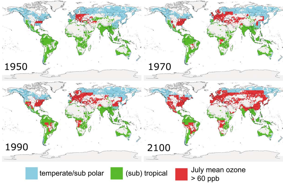
Figure 2. Global forest area where July peak surface O 3 concentration exceeds 60 ppb (from Fowler et al., 1999).
