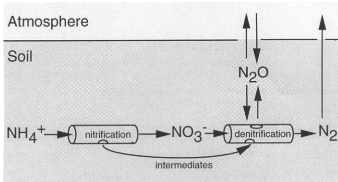
Figure 1. Hole-in-the-pipe model for nitrous oxide dynamics in and transport into or out of soils (Adapted from [4]).
