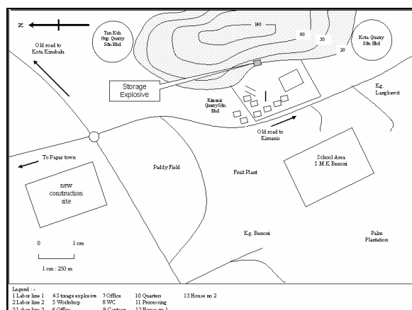
Fig. 1: Quarry and storage explosive location
