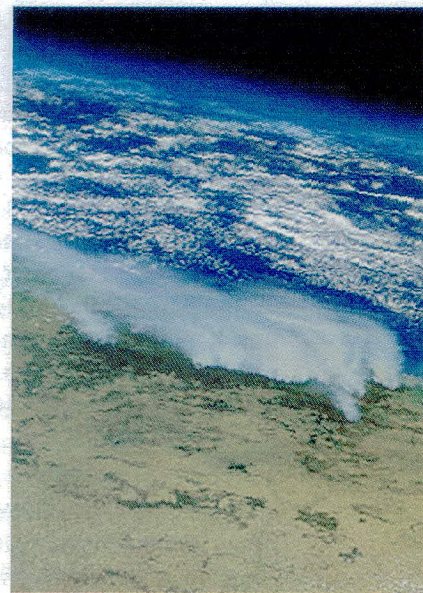
Smoke from fires near Sydney taken by the Sea-Viewing Wide Field-of-view Sensor (Source : Nasa's Earthobservatory)
