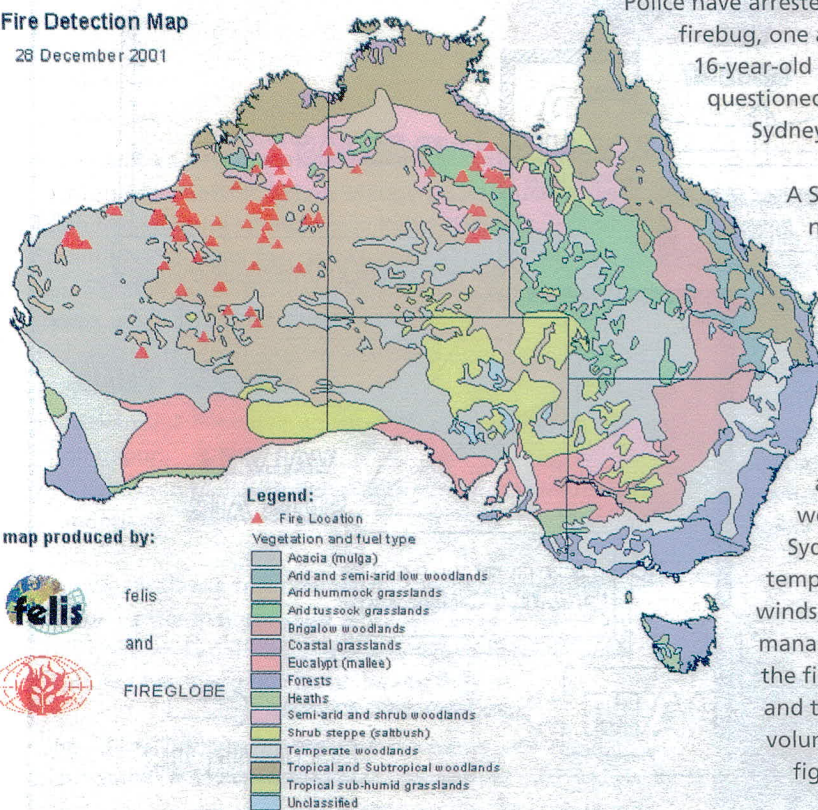
Fire Detection Map for Australia for 28 December 2001 overlaid on a pan-Australian
