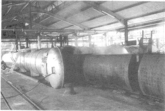
↑ Sterilisation of Fresh Fruit Bunches
