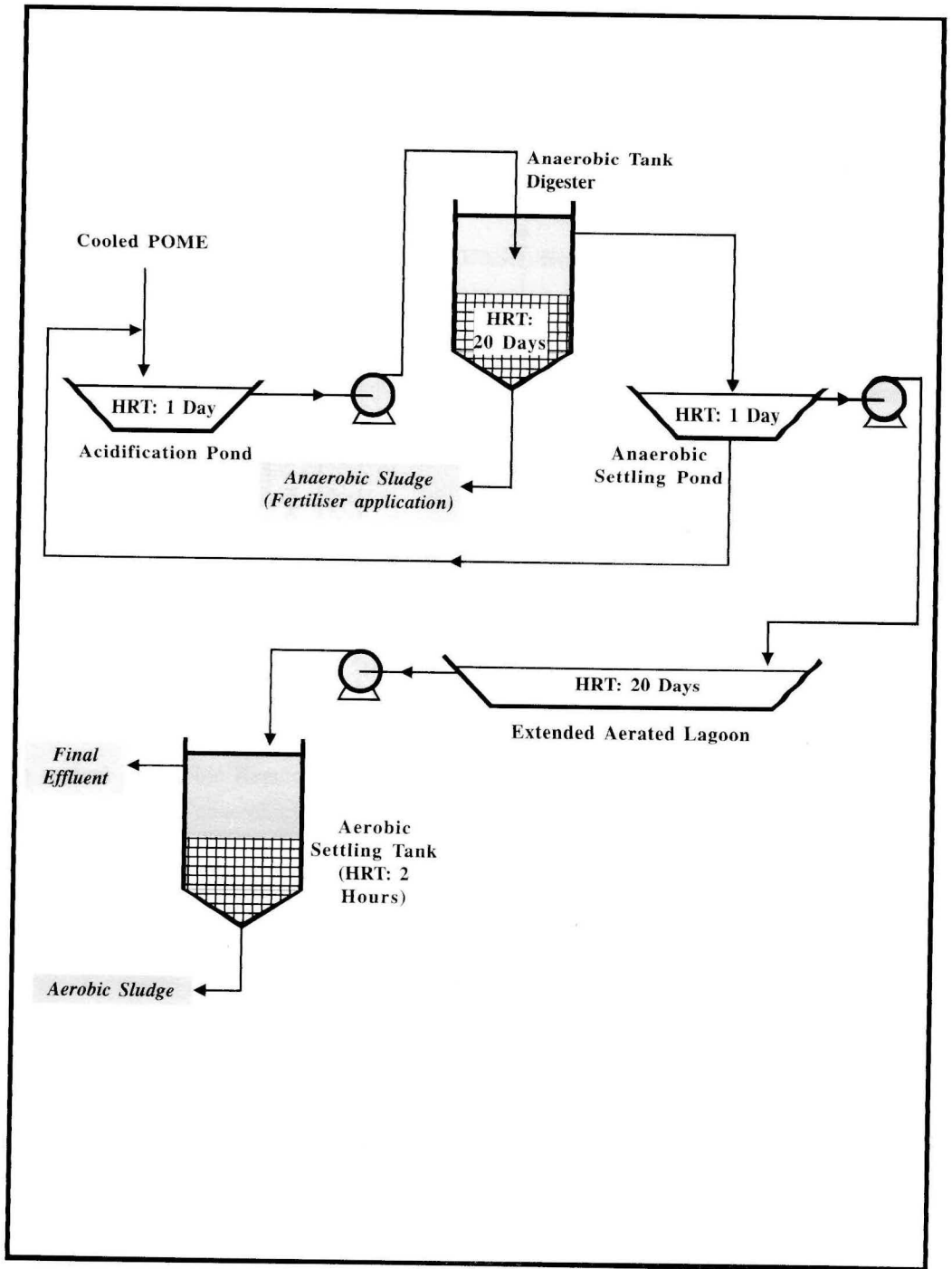
Figure 9: Typical Anaerobic Reactor-cum-Aerated Lagoon System
