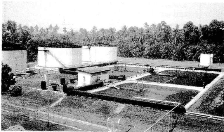
← A Typical Lagoon System
