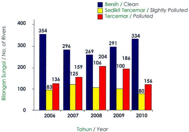
3 (g) : Kualiti Air Sungai Berdasarkan SS Sub-Indeks (2006 - 2010) / River Water Quality Trend based on SS Sub-Index (2006 - 2010)
