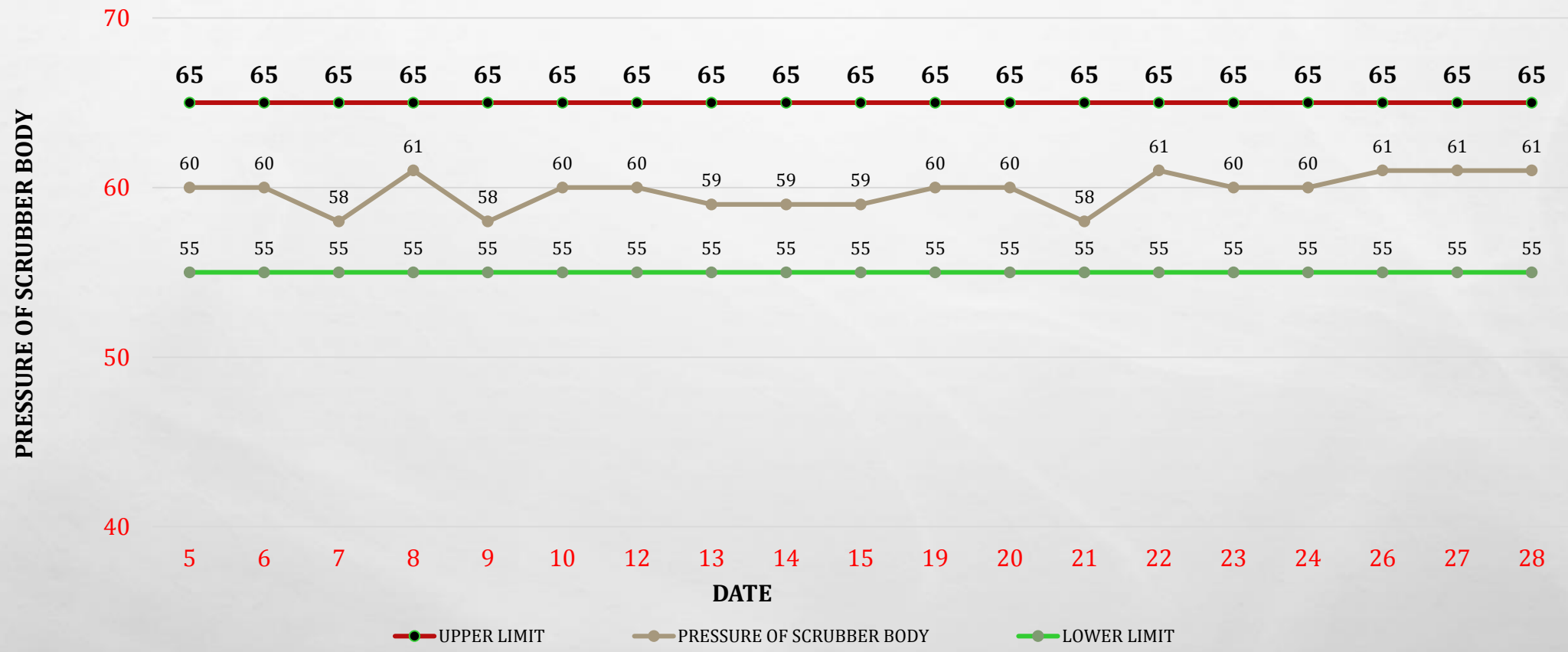
PRESSURE OF SCRUBBER BODY FOR MONTH OF FEBRUARY 2018
