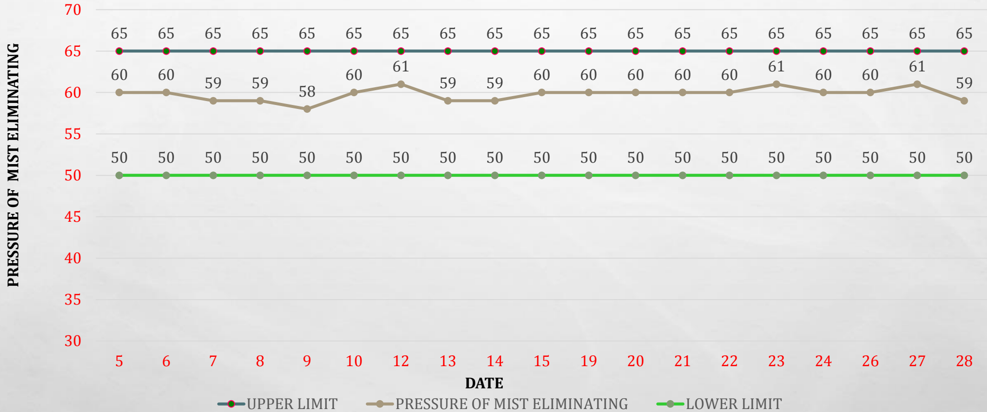
PRESSURE OF MIST ELIMINATING FOR MONTH OF FEBRUARY 2018
