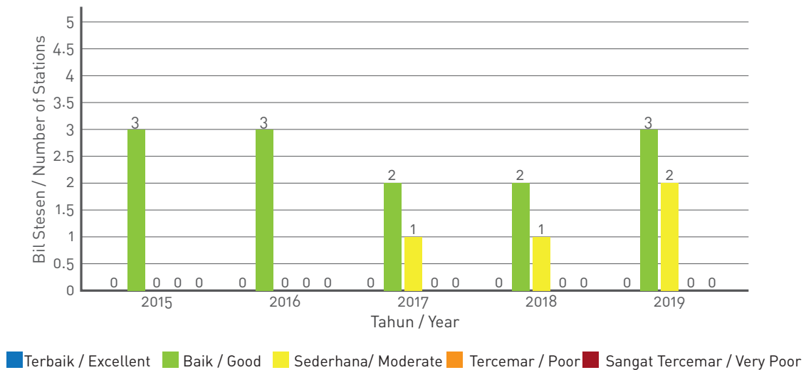
Rajah 3.6: Tren Indeks Kualiti Air Tanah bagi Luar Bandar (2015-2019) Figure 3.6: Trends of Groundwater Quality Index for Rural (2015-2019)
