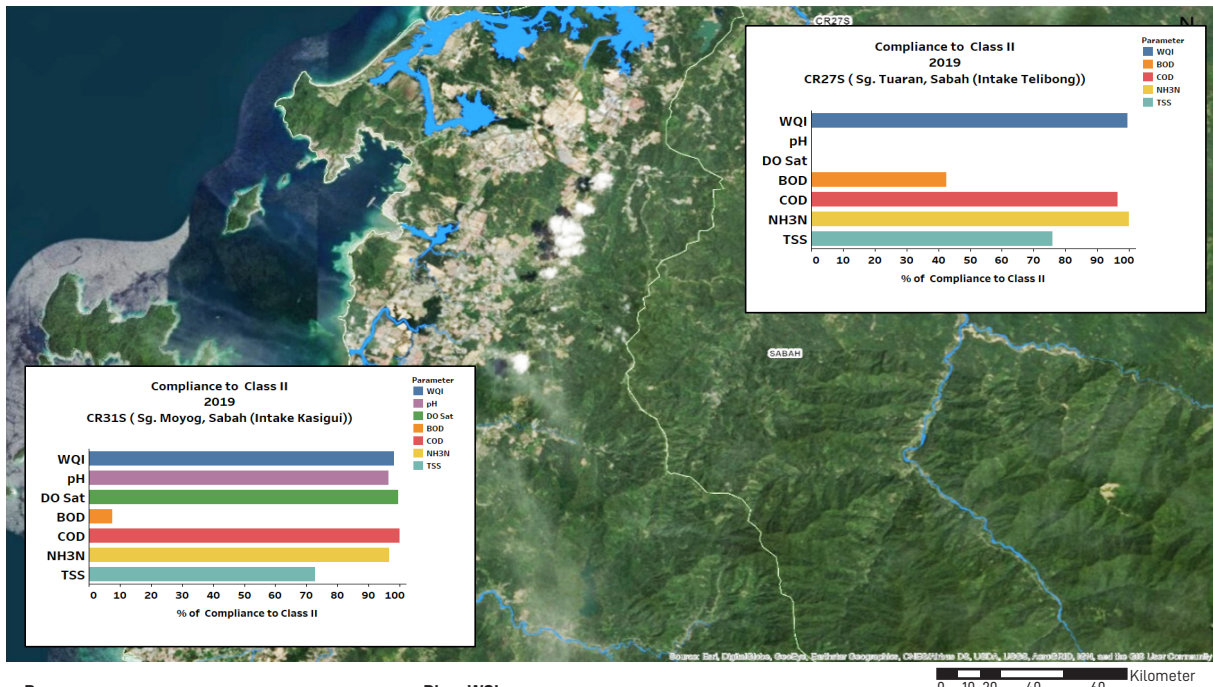
Peratus Pematuhan Kelas II (Sabah) Percentage of Compliance to Class II (Sabah)
