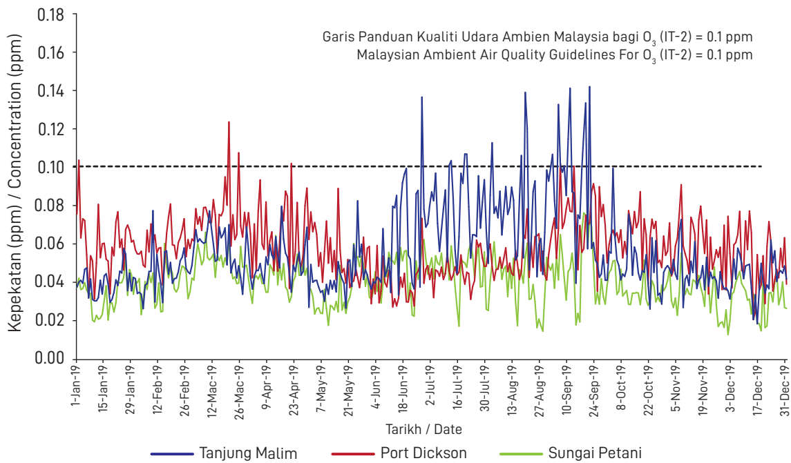
Rajah 1.1(e) : Tren Kepekatan Maksimum Harian Ozon (O 3 ) 1 Jam, Malaysia, 2019 Figure 1.1(e) : Trend of Daily Maximum 1-hour Concentration of Ozone (O 3 ), Malaysia, 2019
