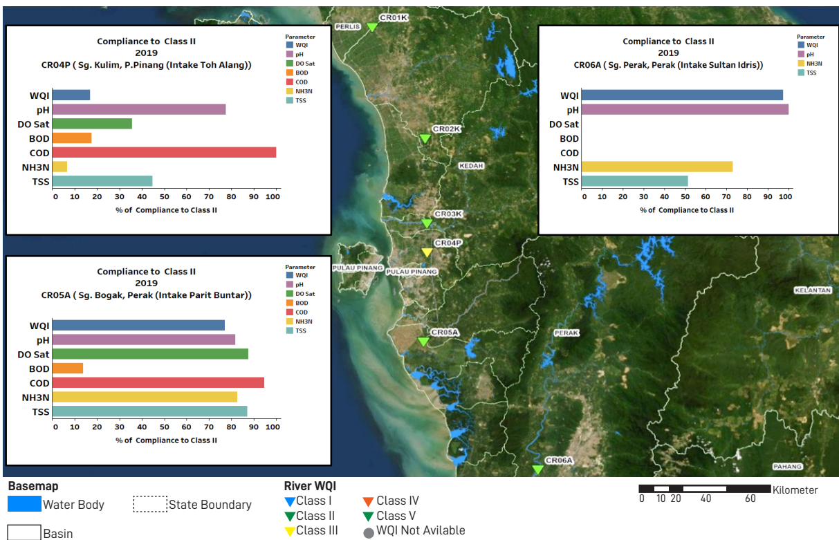
Peratus Pematuhan Kelas II (Utara) Percentage of Compliance to Class II (Northern)
