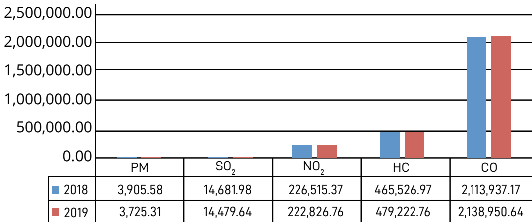
Rajah 5.15 : Beban Pencemar Udara dari Kendaraan Bermotor, 2018 - 2019 Figure 5.15: Air Pollutant Emission Load from Motor Vehicles, 2018 - 2019
