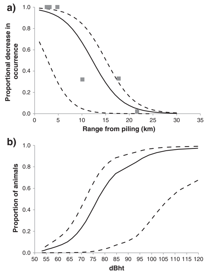
Fig. 5. a) Predicted relationship between range from the Horns Rev II piling operation and the proportional decrease in harbour porpoise occurrence (mean porpoise positive minutes from CPODs (from Brandt et al., 2011)) in the hour after the event; relationship for the line of best fit (deviance = 4.19; d.f. = 1; P < 0.05 ; Intercept = 3.9 (se = 2.77; Range = -0.32 (SE = 0.23)). The best fitted relationship is shown as a solid line. Standard errors were used to provide confidence limits around this relationship. However, because small sample sizes resulted in the upper bound showing almost no variation across the range of distances studied, we instead produced an upper bound for the relationship by weighting the line to include all data points. The lower bound is based upon the standard error of the coefficients. b) The relationship between \text{dB}_{\text{ht}} (harbour porpoise) and the predicted proportion of animals excluded from the area (using the upper, best and lower fitted relationship from Fig. 5a).
