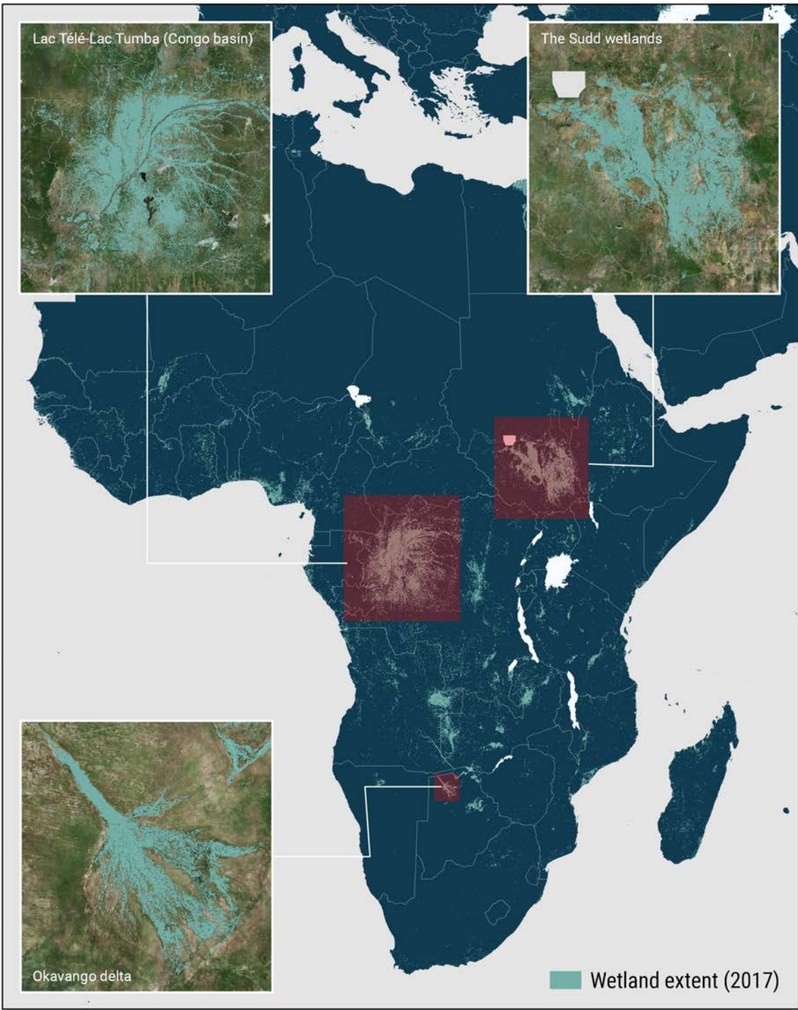
Figure 32. Africa's wetlands
