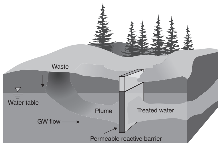
FIGURE 5.3 Permeable reactive barrier. (Adapted from EPA/600/R-98/125.)
