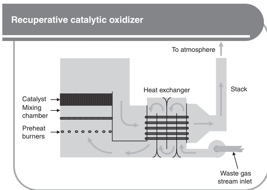
FIGURE 6.8 Schematic representation of a catalytic incinerator. (Adapted from EPA Technology Transfer Network. http://cfpub.epa.gov/oarweb/mkb/conttechnique.cfm?ControllID=10. )
