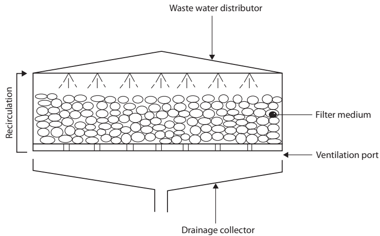
FIGURE 7.6 Schematic representation of conventional trickling filter. (Permission granted courtesy of Laxmi Publications Pvt. Ltd.)
