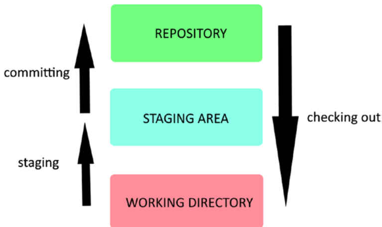
Figure 6-1. The relationship between the three states of Git
