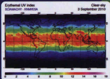
UV exposure on Earth
