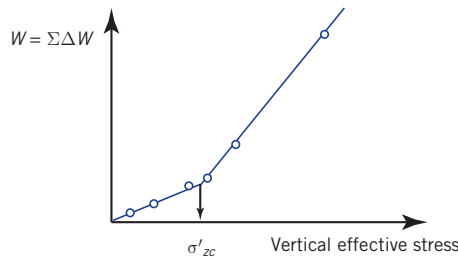
Figure 7.15 Determination of the past maximum vertical effective stress using the strain energy method.
