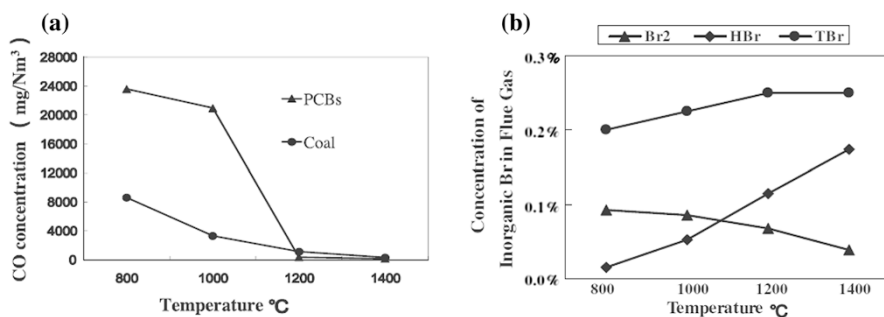
Fig. 3 Effects of temperature on CO emission (a) and HBr/ \text{Br}_2 emission (b) (excess air factor = 1.3, high temperature zone residence time = 0.25 s)
