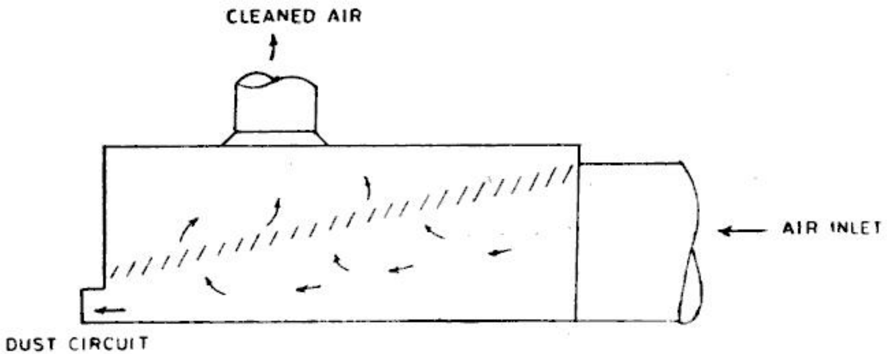
Fig. 13.3 Louvre dust collector
