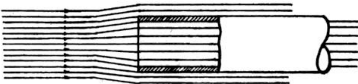
(b) FLOW RATE LESS THAN ISOKINETIC RATE
