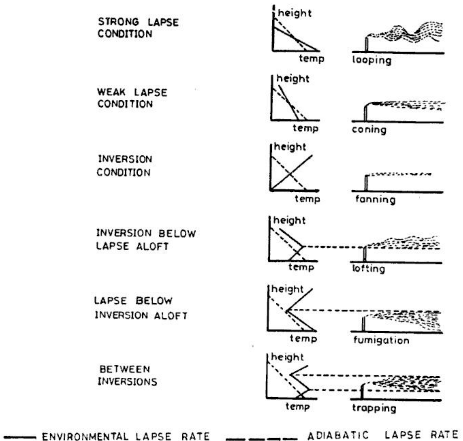
Fig. 3.5 Types of plume behaviour
