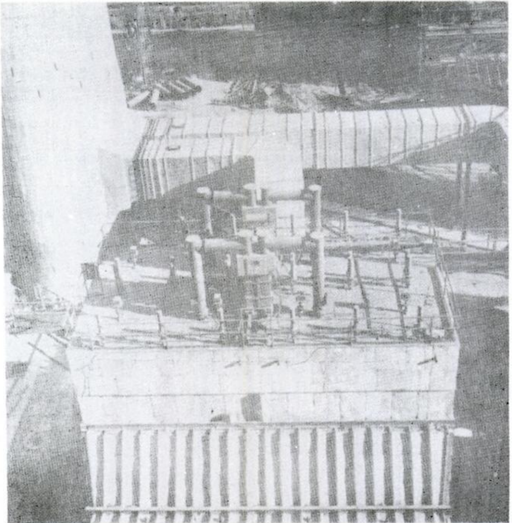
Top view of an ESP showing outlet ducting to the stack, TR sets and IIT bus duct and rappers. (Courtesy: VOLTAS LTD.)
