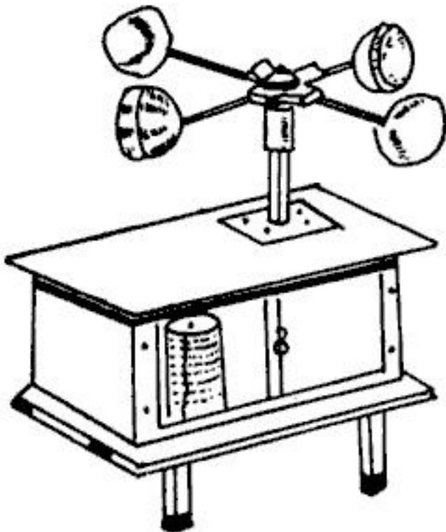
Fig. 3.2 Wind speed recorder
