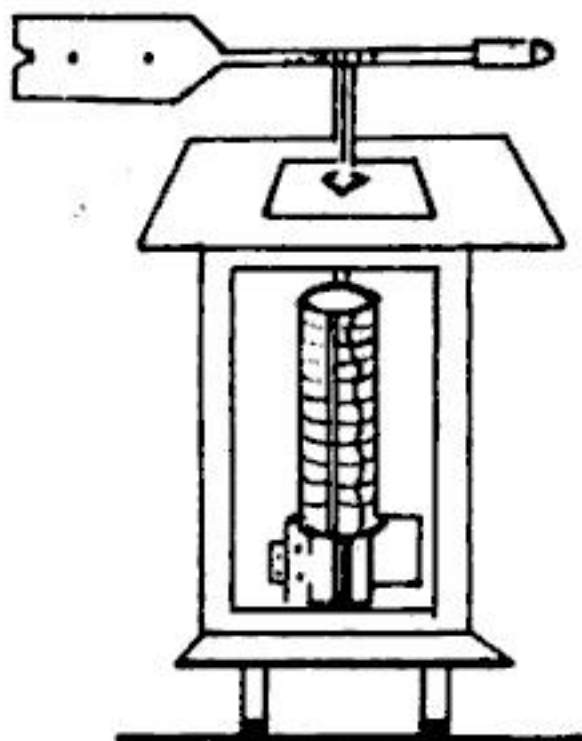
Fig. 3.1 Wind direction recorder
