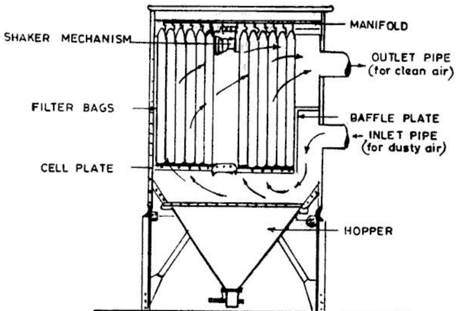
Fig. 13.8 Bag house filter
