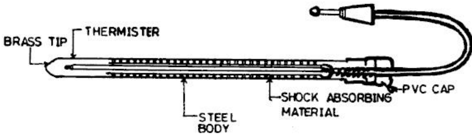
Fig. 3.3 Probe details
