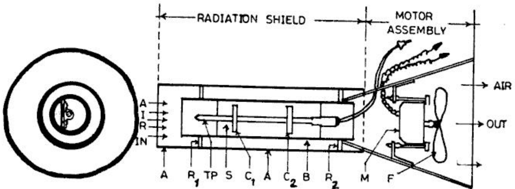
Fig. 3.4 Motor aspirated radiation shielded temperature sensor
