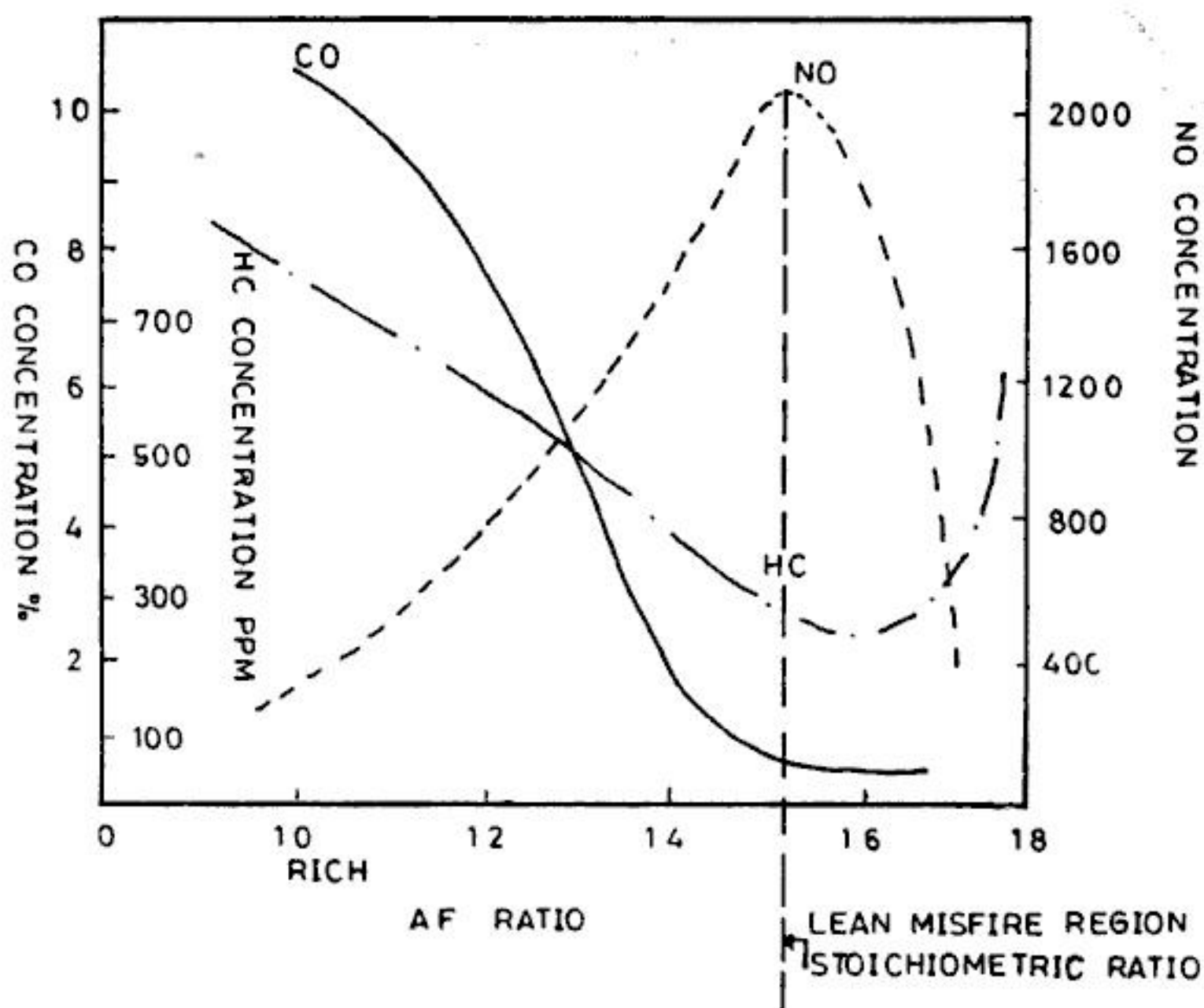
Fig. 11.3 Effect of AF Ratio
