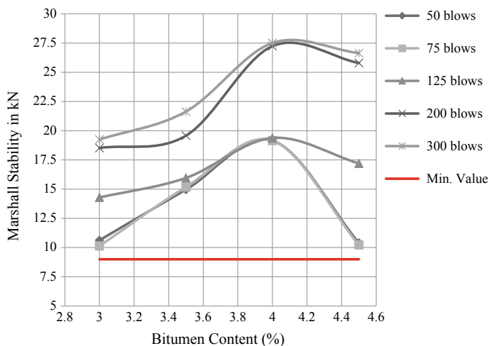
Fig. 5 Stability value characterized by Bitumen content
