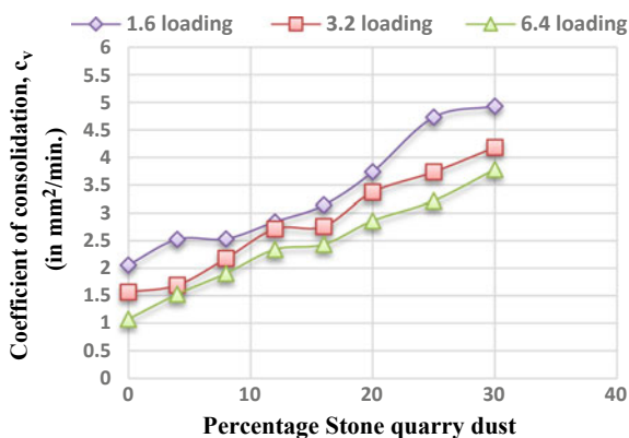
Fig. 7 Variation of coefficient of consolidation with percentage of stone quarry dust
