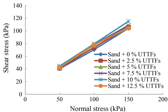
Fig. 5 Variation of shear stress with normal stress for UTFs
