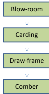
Fig. 1 Material sequence at spinning preparatory
