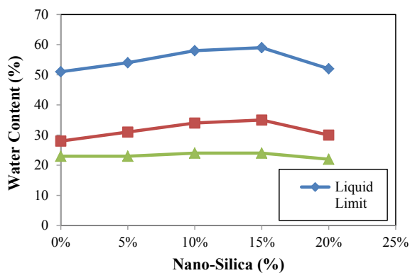
Fig. 1 Effect of nano-silica on Atterberg limits
