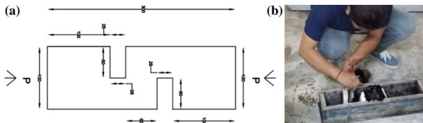
Fig. 2 a Schematic shear test specimen and b oiling on mould
