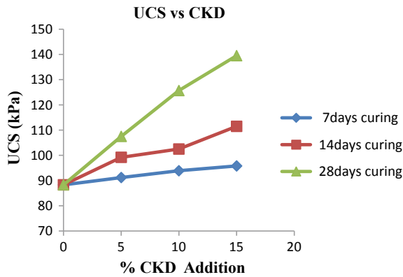
Fig. 3 Influence of % CKD addition on the UCS of clay cured at 7, 14 and 28 days
