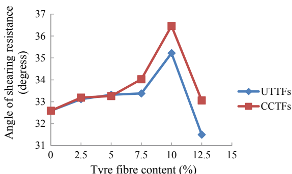
Fig. 9 Variation of angle of shearing resistance with tyre fibre content for UTFs and CCTFs
