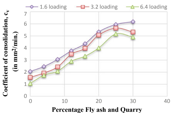
Fig. 8 Variation of coefficient of consolidation with percentage of fly ash stone quarry dust
