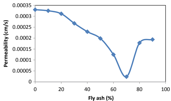
Fig. 2 Permeability versus percentage of fly ash
