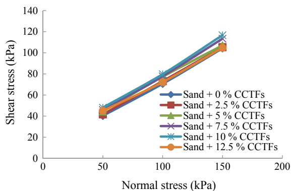
Fig. 6 Variation of shear stress with normal stress for CCTFs
