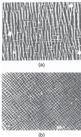
Figure 4.15 The nanostructure of Alnico 8 after isothermal heat treatment in a magnetic field for 9 h at 800 °C: (a) view perpendicular to the direction of the applied field, (b) view along the direction of the applied field. The microstructure has a periodicity of approximately 32 nm. After R. C. O'Handley, Modern Magnetic Materials: Principles and Applications , Wiley, New York, 2000, p. 481
