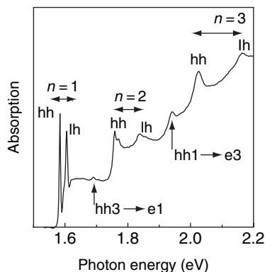
Figure 3.33 Low-temperature absorption spectrum of a 40-period GaAs–AlAs multiple quantum well structure with 7.6 nm wide wells. The most intense features result from transitions between the n th ( n = 1, 2, 3 ) confined light hole (lh) and heavy (hh) hole states and identical index electron states. In addition, two weaker transitions are observed between the first and third heavy hole and electron states ( hh3 \rightarrow e1 and hh1 \rightarrow e3 ). Data reproduced by permission of Taylor and Francis Ltd from A. M. Fox, Contemp. Phys. 37 , 111 (1996)
