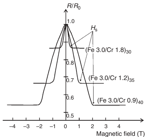
Figure 4.18 Normalized resistance ( R/R_0 ) as a function of applied magnetic field for an Fe/Cr multilayer. The notation (\text{Fe } x/\text{Cr } y)_z denotes a stack of z bilayers of x nm of iron and y nm of chromium. H_s is the saturation field as defined in the text. Redrawn with permission after B. Heinrich and J. A. C. Bland, Ultrathin Magnetic Structures , Vol. I, Springer-Verlag, Berlin, 1994, p. 98. Copyright 1994 Springer-Verlag
