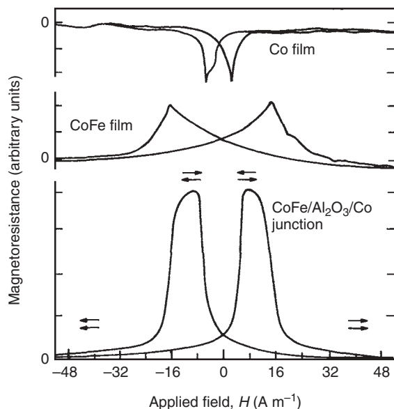
Figure 4.23 Anisotropic magnetoresistance in each individual CoFe and Co electrode and the junction magnetoresistance in \text{CoFe}/\text{Al}_2\text{O}_3/\text{Co} spin tunnel junction versus applied field. After R. C. O'Handley, Modern Magnetic Materials: Principles and Applications , Wiley, New York, 2000, p. 607. Copyright 2000 with permission of John Wiley & Sons Inc.
