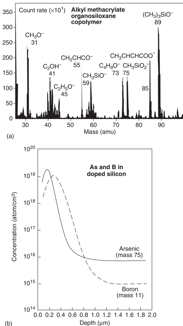
Figure 2.26 Schematic diagram of (a) a static SIMS spectrum from a copolymer film and (b) an example of a depth profile measured using dynamic SIMS
