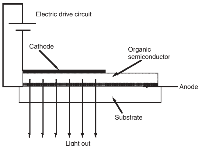
Figure 6.15 OLED architecture
