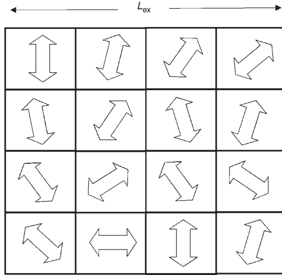
Figure 4.6 A schematic illustration of a nanostructured soft ferromagnet. Each square represents one grain, and the block arrows represent the direction of magnetization within each grain. L_{\text{ex}} is the exchange length
