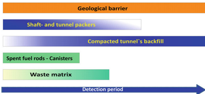
Fig. 3.3 Scheme of the temporal effect of various barriers in the repository system, in the detection period of one million years (not to scale)
