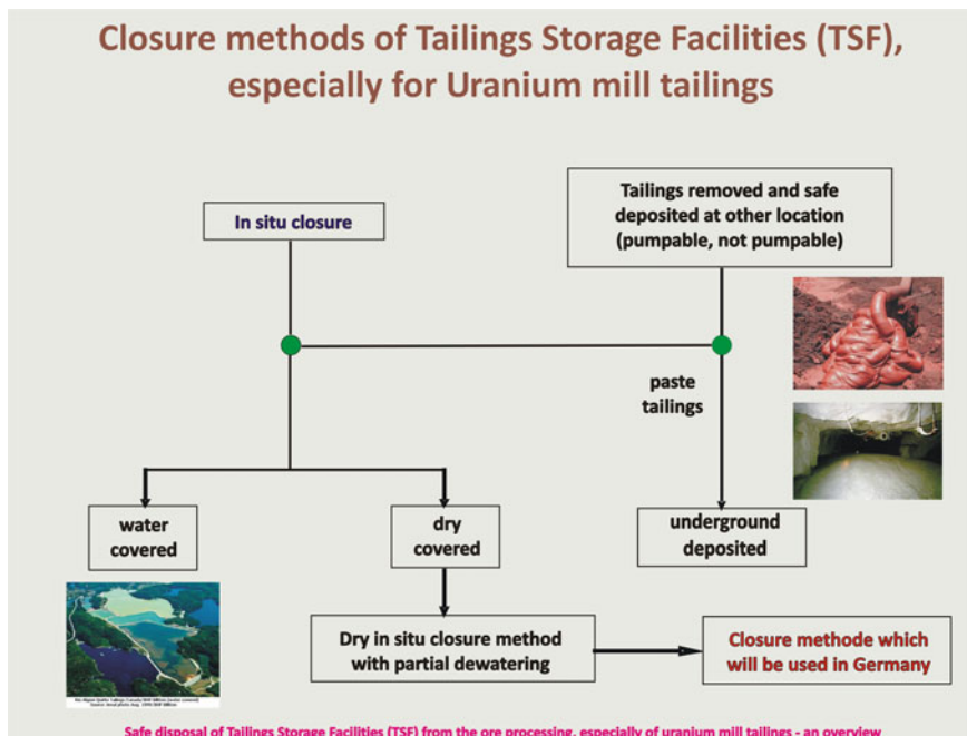
Fig. 5.11 Closure methods of Uranium mill tailings ponds, location-dependent, also from the different climatic conditions
