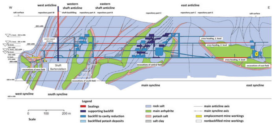
Fig. 6.10 Schematic section through the backfilled and closed pit cavities of ERA Morsleben. Source Federal Office for Radiation Protection [17]
