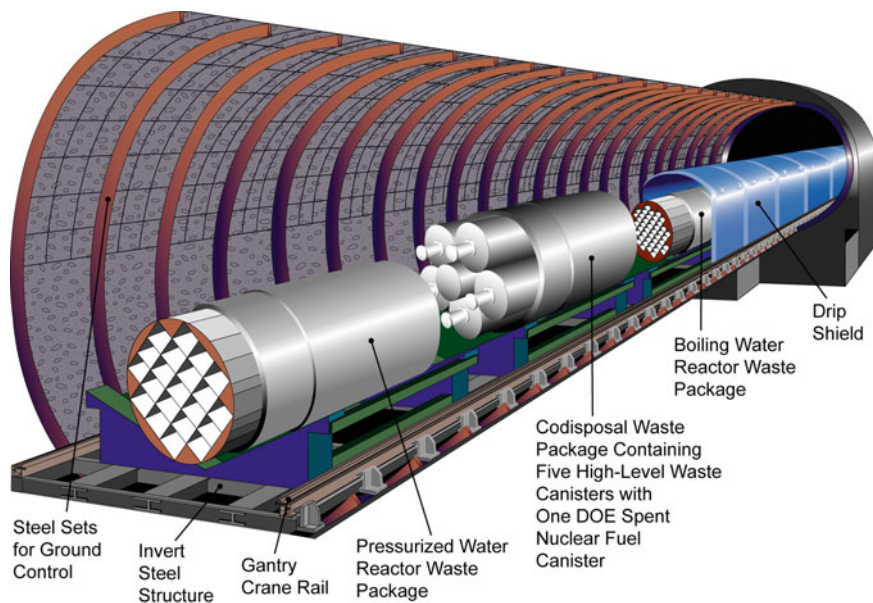
Fig. 7.9 Types of waste packages depending on the type of waste. Source US Department of Energy (DOE)
