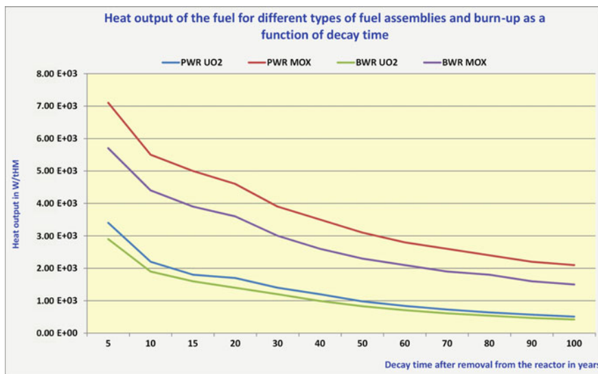
Fig. 7.1 Heat output of fuel for different types of fuel elements and burn-up in dependence of the decay time, according Table 7.5 and [11]
