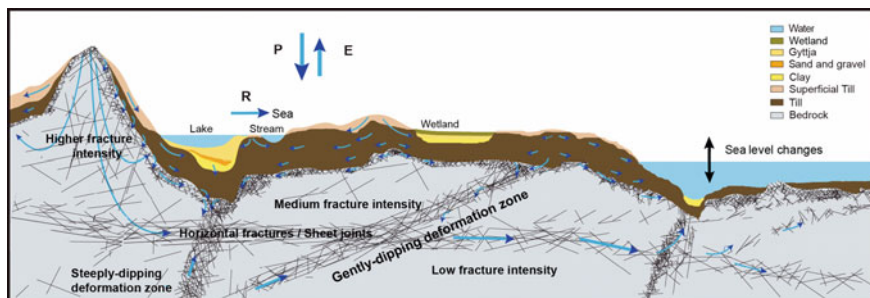
Fig. 7.17 Geological Barrier-principle. Source Föllin et al. [51]; SKB AB, public domain P = precipitation, E = evapotranspiration, R = runoff
