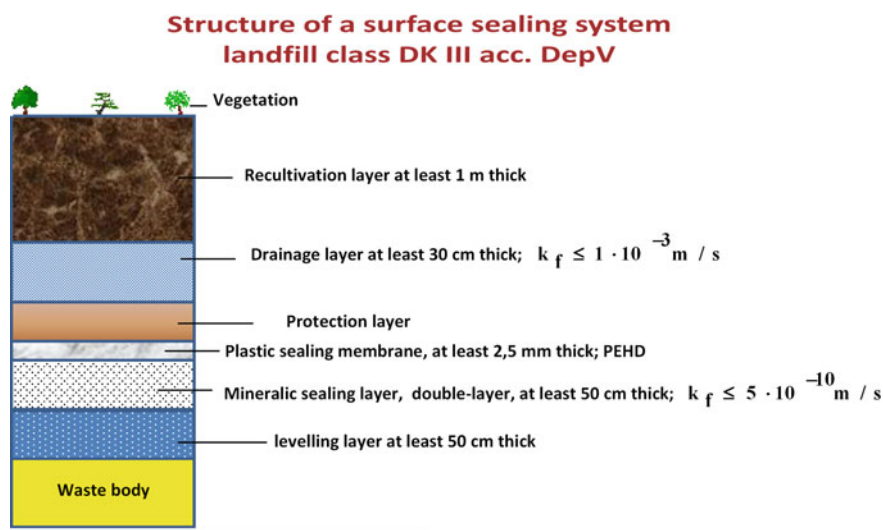
Fig. 4.5 Surface sealing for landfill DK III acc. to DepV; pursuant to Table 4.4
