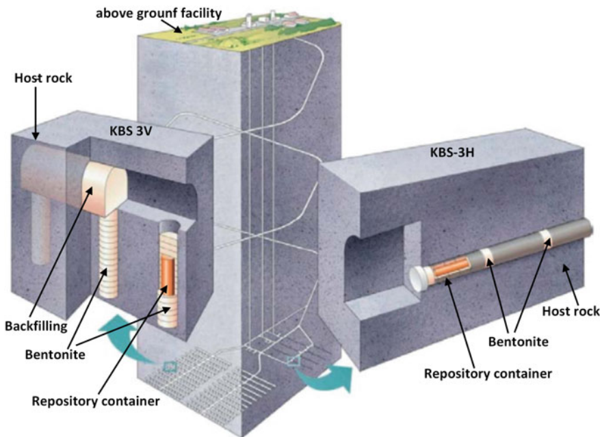
Fig. 7.20 Vertical and horizontal container emplacement and the envisaged geotechnical barriers in Olkiluoto's long-term safety concept. Source © SKB AB; public domain
