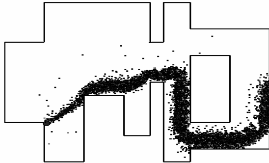
Fig. 10.10 Particle dispersion pattern case 3.
