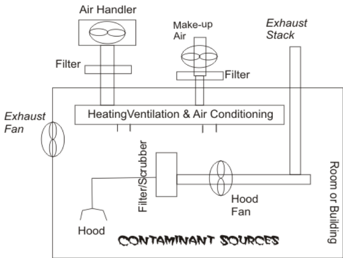
Fig. 1.1 Schematic of a typical ventilation system.
