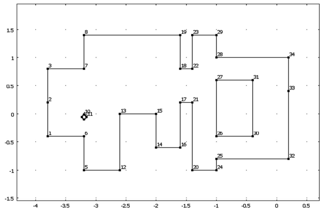
Fig. B.1.2 Grid vertices for 2-D office configuration for COMSOL MultiPhysics software.
