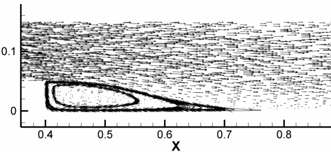
Fig. 9.16 Vectors on refined grid for flow over a 2-D backward-facing step at Re = 42,000 .
