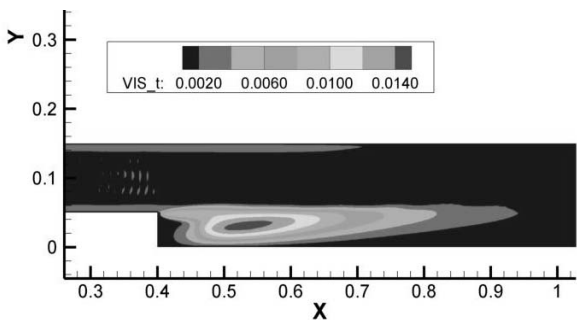
Fig. 9.18 Re = 42,000 : Effective viscosity distribution behind step.
