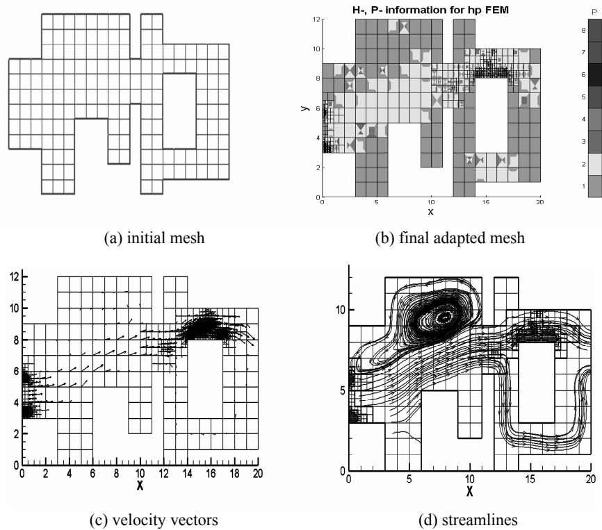
Fig. 7.32 FEM h-p adaptation simulation for office complex.
