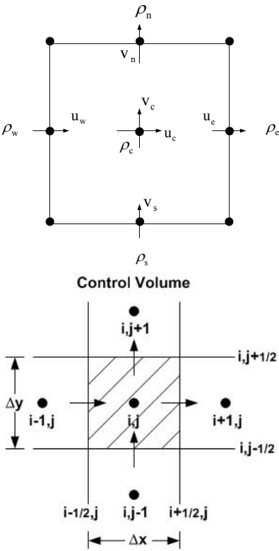
Fig. 7.6 Discretization of a finite volume.
