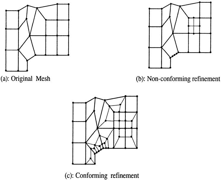
Fig. 7.27 Mesh refinement
