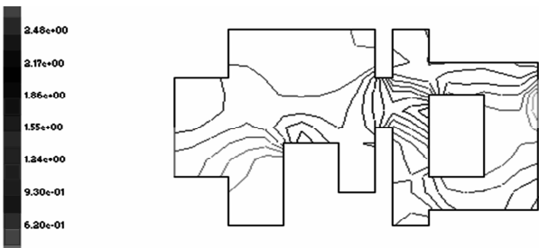
Fig. 7.10 Isobars from FVM solution for the office complex.
