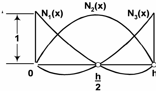
Fig. 7.13 One-dimensional quadratic element and shape functions.
