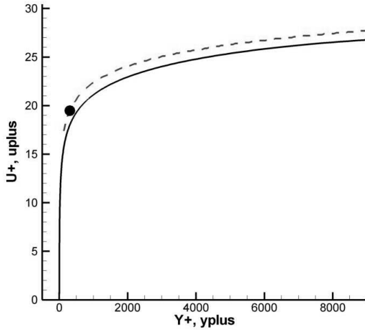
Fig. 9.15 U^+ vs. Y^+ for developed flow. Solid line from Wilcox's Pipe Flow Program (2006) k - \omega solution for duct flow vs. FEM predictions, Re = 13,750 .
