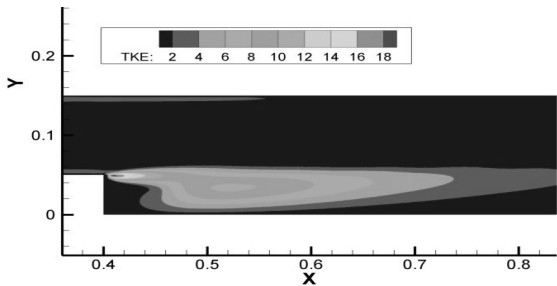
Fig. 9.19 Re = 42,000 : Turbulent kinetic energy distribution behind step.
