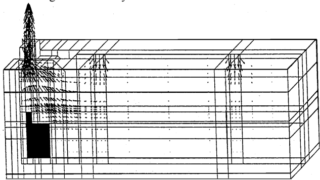
Fig. 7.34 Velocity vectors in side view of kitchen.
