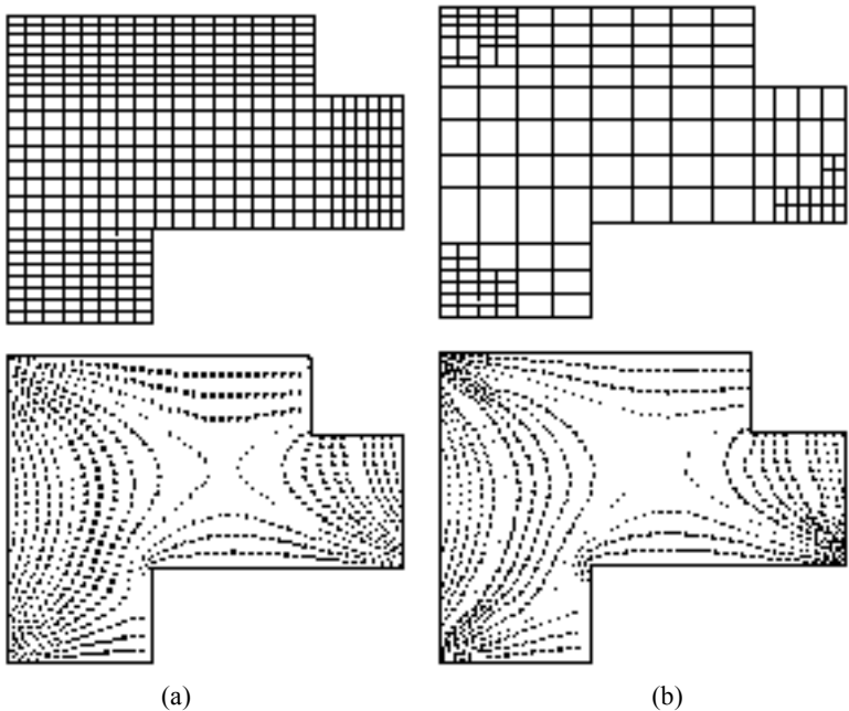
Fig. 8.22 FEM solutions (a) meshless (on FEM fine mesh) and (b) adapted mesh.
