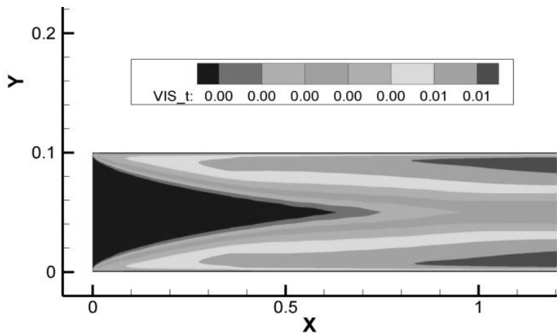
Fig. 9.10 Turbulent eddy viscosity.
