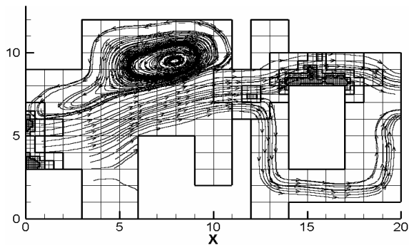
Fig. 10.7 Streamlines.
