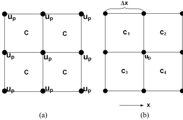
Fig. 8.8 Two-dimensional PIC mesh.
