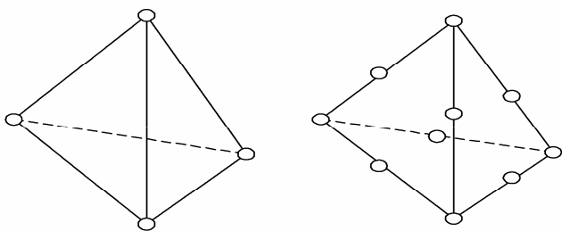
Fig. 7.21 Linear and quadratic tetrahedral elements.
