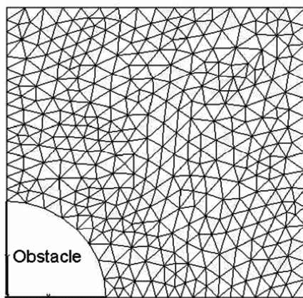
Fig. 7.23 Example of an unstructured two-dimensional grid.
