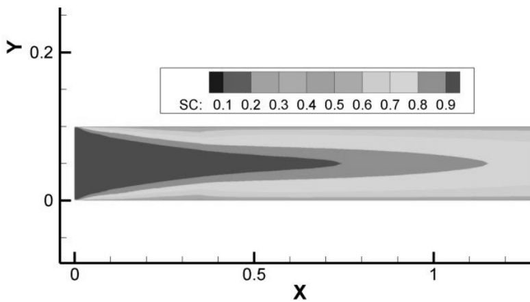
Fig. 9.13 Species concentration.
