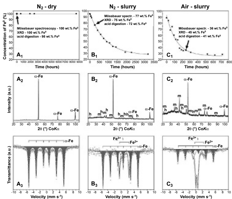
Figure 6.8 Stability of nZVI in air and \text{N}_2 conditions in sequence of decreasing nZVI stability. Weigh percentages of measured \text{Fe}^0 (i.e., \alpha -Fe) as a function of the exposure time of nZVI to its storage environment. Characteristic X-ray powder diffraction patterns (m—magnetite/maghemite; h—hematite) and ^{57}\text{Fe} Mössbauer spectra of quality sufficient for nZVI evaluation and collected at reasonable time for routine analysis. Data partly adapted with permission from Ref. [28]. Copyright 2014 American Chemical Society.
