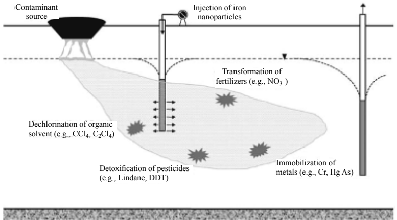
Figure 1.2 Nanoscale iron particles for in situ remediation. Reprinted by permission from Springer Nature: Kluwer Academic Publishers, Journal of Nanoparticle Research , Ref. [5], Copyright 2003.
