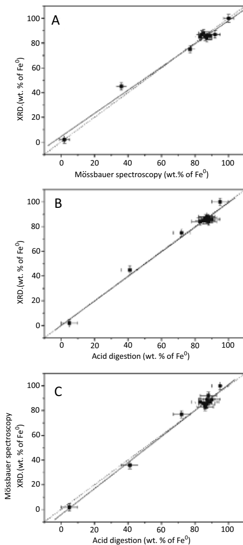
Figure 6.10 Comparison of results of XRD, Mössbauer spectroscopy, and acid digestion measured on a broad range of Fe 0 /Fe tot ratios. The dotted line represents the 1:1 ratio.
