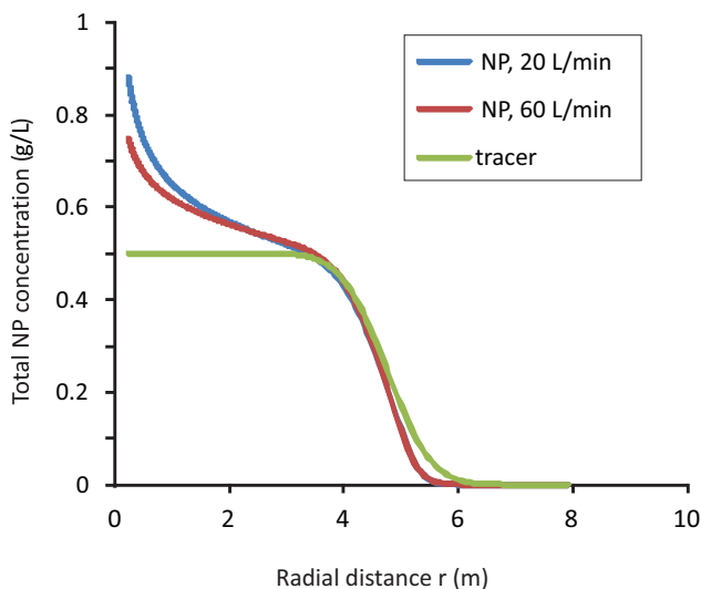
Figure 5.7 Total (suspended + deposited) concentration of ferrihydrite NPs and of a tracer as a function of the radial distance r from the injection well.
