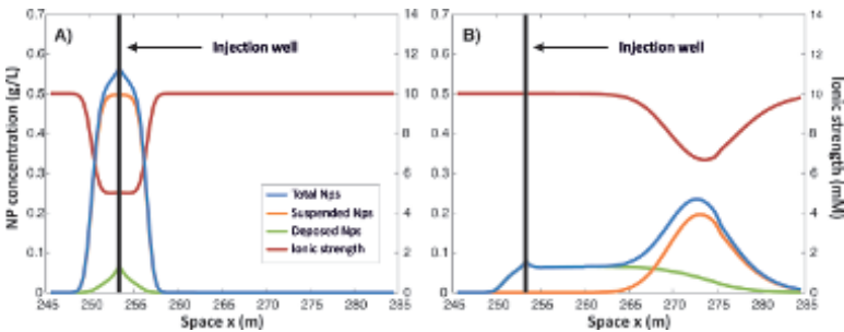
Figure 5.9 Total (suspended + deposited) NP concentration, deposited NP concentration, and ionic strength profile along the section S-S at the end of the injection (A) and after 10 days (B).
