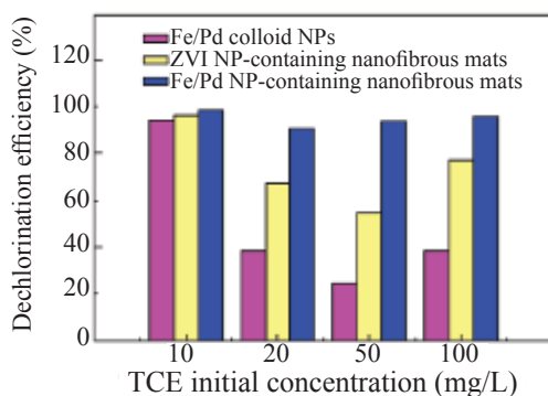
Figure 11.6 Removal efficiency of TCE by Fe/Pd colloidal NPs, ZVI NP- and Fe/Pd NP-containing nanofibrous mats with different initial TCE concentrations. The reaction time was 1.5 h. Reprinted from Ref. [60], Copyright 2012, with permission from Elsevier.
