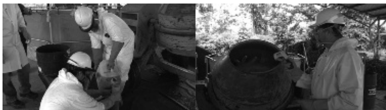
Figure 7.10 Dosage of reactants (left) and control of temperature (right).
