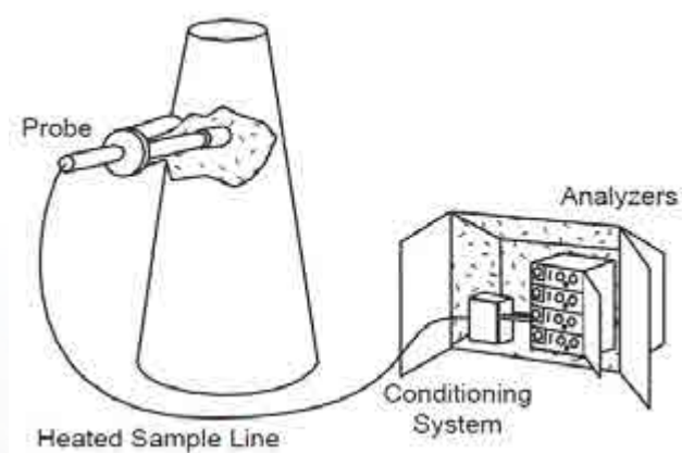
Figure 3.1 Example of Extractive CEMS (source : USEPA 1 )
