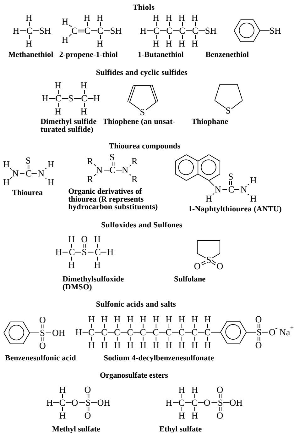
Figure 29.12. Examples of organosulfur compounds.
