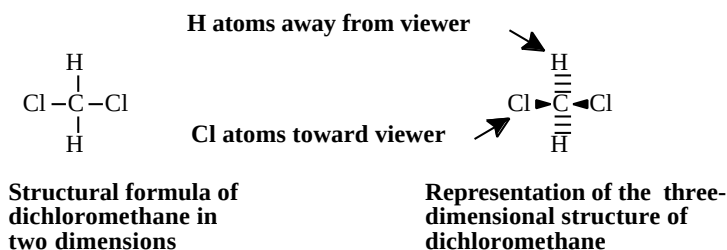
Figure 29.1. Structural formulas of dichloromethane, \text{CH}_2\text{Cl}_2 ; the formula on the right provides a three-dimensional representation.
