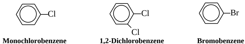
Figure 29.10. Some example organohalide compounds.
