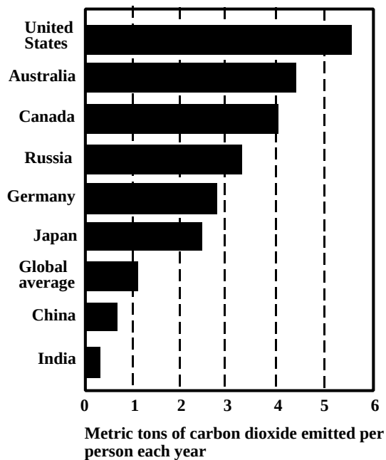
Figure 14.2. Per capita emissions of carbon dioxide. Rapid industrialization of high-population countries, particularly China and India, can be expected to add much larger quantities of carbon dioxide to the atmosphere in the future.
