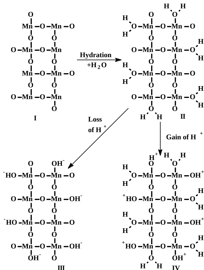
Figure 5.5. Acquisition of surface charge by colloidal \text{MnO}_2 in water. Anhydrous \text{MnO}_2 (I) has two O atoms per Mn atom. Suspended in water as a colloid, it binds to water molecules to form hydrated \text{MnO}_2 (II). Loss of \text{H}^+ from the bound \text{H}_2\text{O} yields a negatively charged colloidal particle (III). Gain of \text{H}^+ by surface O atoms yields a positively charged particle (IV). The former process (loss of \text{H}^+ ion) predominates for metal oxides.
