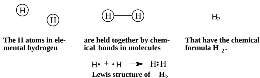
Figure 28.5. Molecule and Lewis formula of \text{H}_2 .
