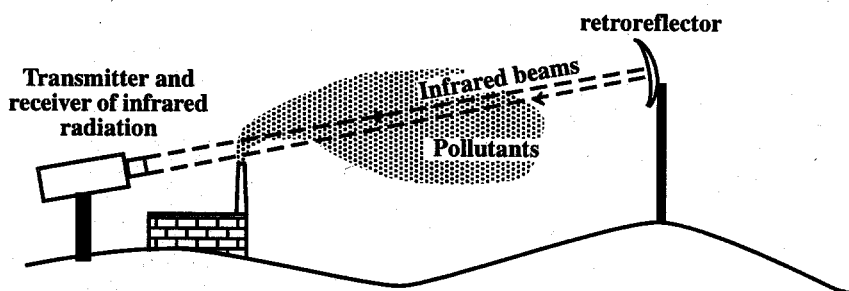
Figure 26.9. FTIR system for remote sensing of air pollutants.
