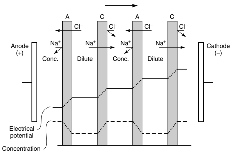
Figure 10.7 Schematic of the concentration and potential gradients in a well-stirred electrodialysis cell
