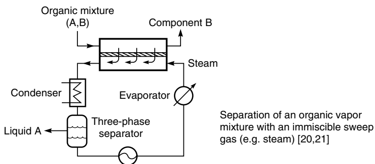
Figure 4.15 Sweep gas systems proposed for industrial processes
