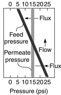
Figure 6.14 Backflushing of membrane modules by closing the permeate port. This technique is particularly applicable to capillary fiber modules
