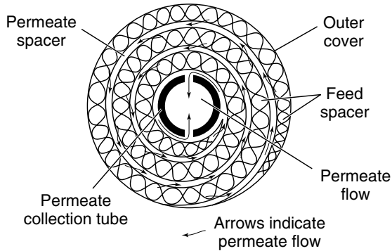
Figure 3.42 Exploded view and cross-section drawings of a spiral-wound module. Feed solution passes across the membrane surface. A portion passes through the membrane and enters the membrane envelope where it spirals inward to the central perforated collection pipe. One solution enters the module (the feed) and two solutions leave (the residue and the permeate). Spiral-wound modules are the most common module design for reverse osmosis and ultrafiltration as well as for high-pressure gas separation applications in the natural gas industry
