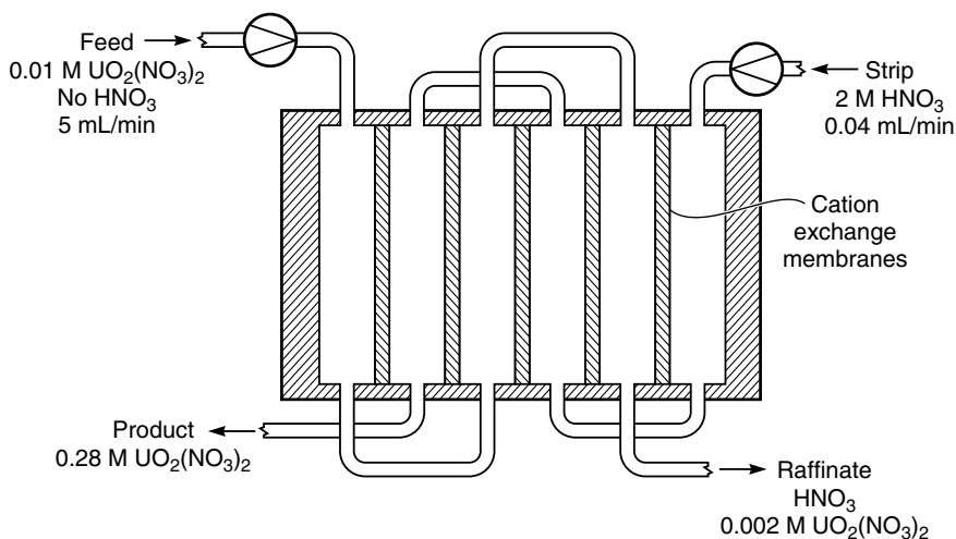
Figure 13.3 Illustration of a Donnan dialysis experiment to separate and concentrate uranyl nitrate, \text{UO}_2(\text{NO}_3)_2 , after Wallace [5]
