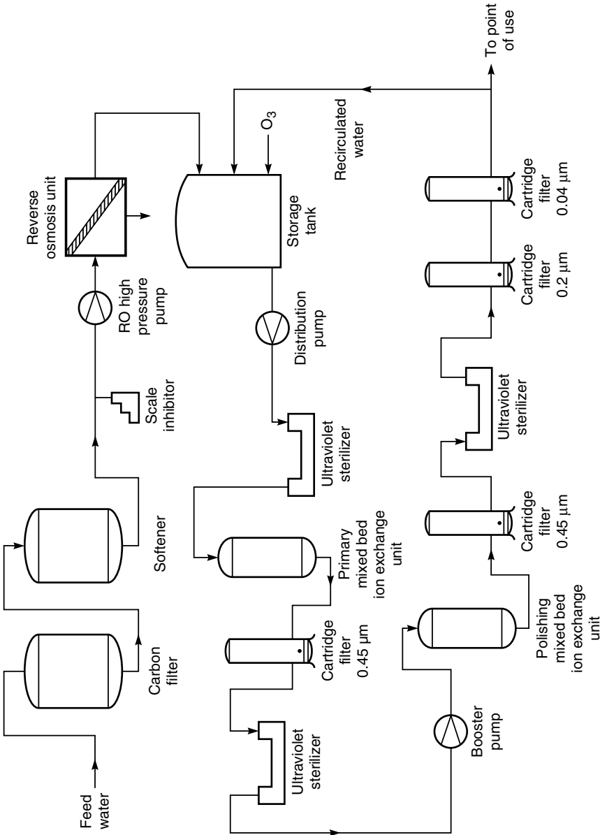
Figure 5.26 Flow schematic of an ultrapure water treatment system [54]
