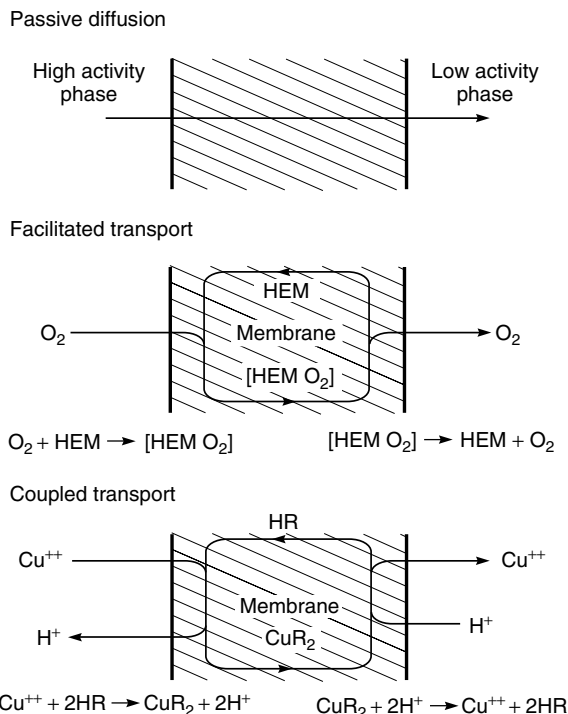
Figure 11.1 Schematic examples of passive diffusion, facilitated transport and coupled transport. The facilitated transport example shows permeation of oxygen across a membrane using hemoglobin as the carrier agent. The coupled transport example shows permeation of copper and hydrogen ions across a membrane using a reactive oxime as the carrier agent
