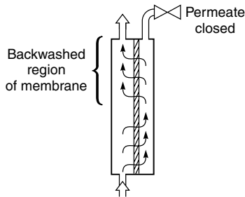
(c) Reverse flow back flushing
