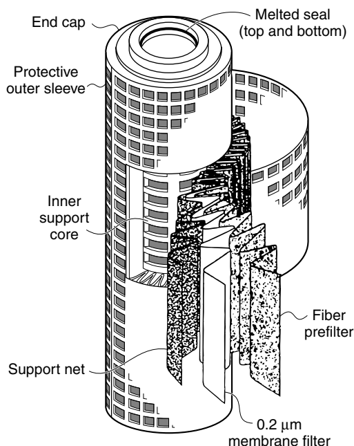
Figure 7.11 Cut-away view of a simple pleated cartridge filter. By folding the membrane a large surface area can be contacted with the feed solution producing a high particle loading capacity. (From Membrana product literature)
