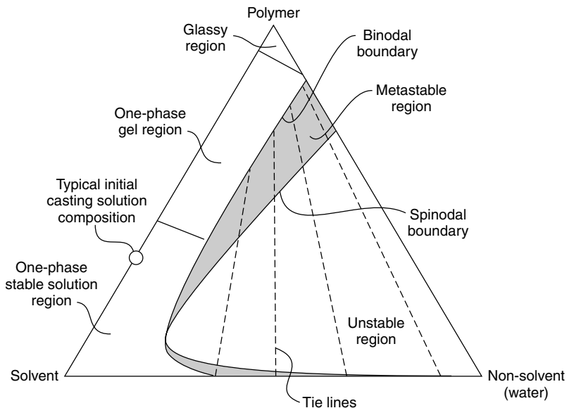
Figure 3.11 Schematic of the three-component phase diagram often used to rationalize the formation of water-precipitation phase separation membranes
