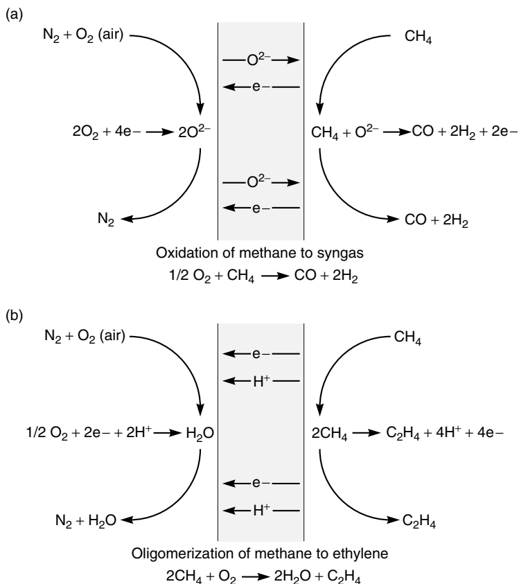
Figure 13.21 Use of ion-conducting ceramic membranes in a membrane reactor to produce (a) syngas ( \text{CO} + \text{H}_2 ) and (b) ethylene
