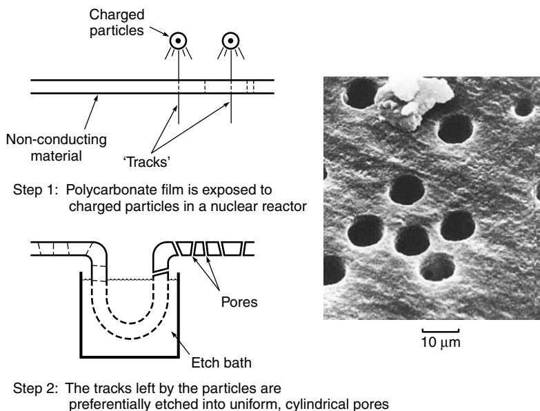
Figure 3.4 Diagram of the two-step process to manufacture nucleation track membranes [4] and photograph of resulting structure. (Photograph courtesy of Whatman plc, Maidstone, Kent, UK)
