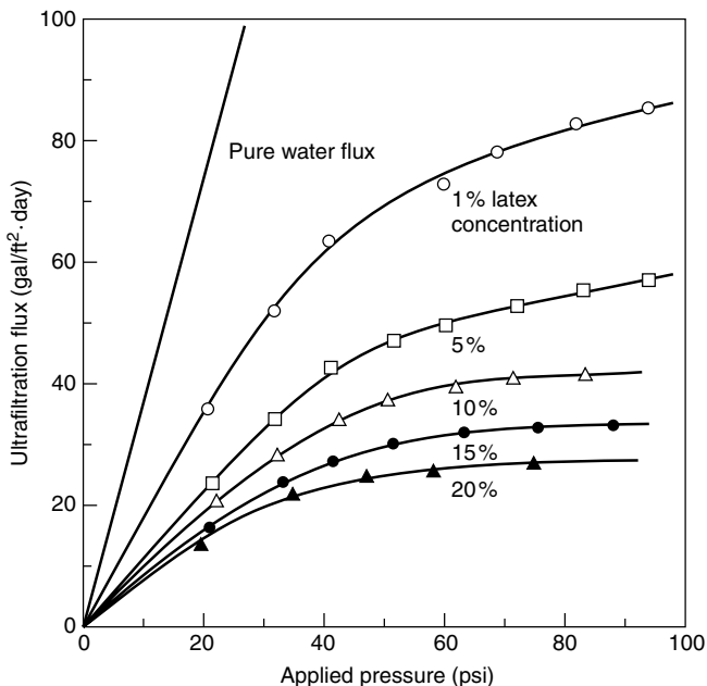
Figure 6.8 The effect of pressure on membrane flux for styrene-butadiene polymer latex solutions in a high-turbulence, thin-channel test cell [13]
