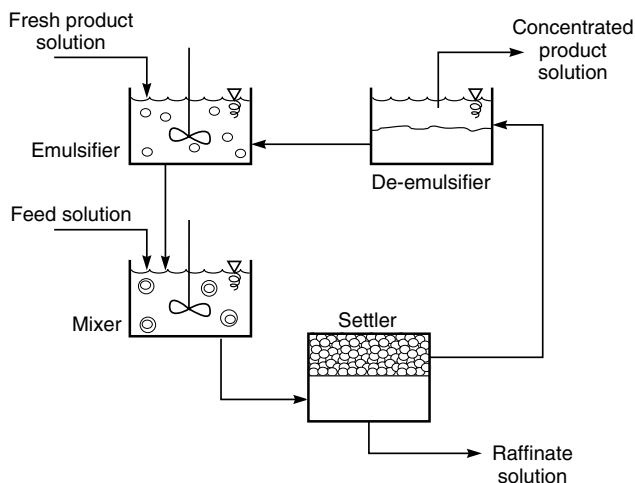
Figure 11.14 Flow diagram of a liquid emulsion membrane process
