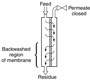
(c) Reverse flow back flushing
