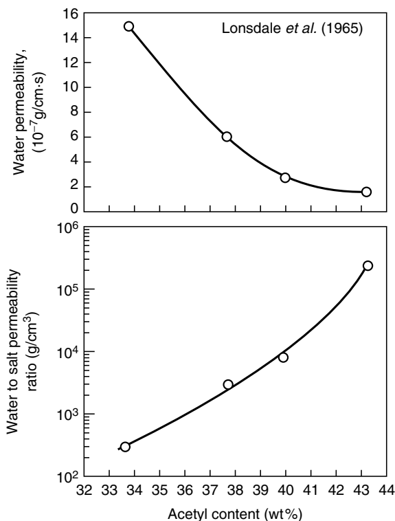
Figure 5.4 Permeabilities of cellulose acetate to water and sodium chloride as a function of acetyl content at 25 °C. Data from Lonsdale et al. [20]
