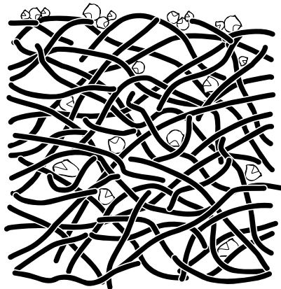
Figure 7.3 Surface scanning electron micrograph and schematic comparison of nominal 0.45- \mu\text{m} screen and depth filters. The screen filter pores are uniform and small and capture the retained particles on the membrane surface. The depth filter pores are almost 5–10 times larger than the screen filter equivalent. A few large particles are captured on the surface of the membrane, but most are captured by adsorption in the membrane interior
