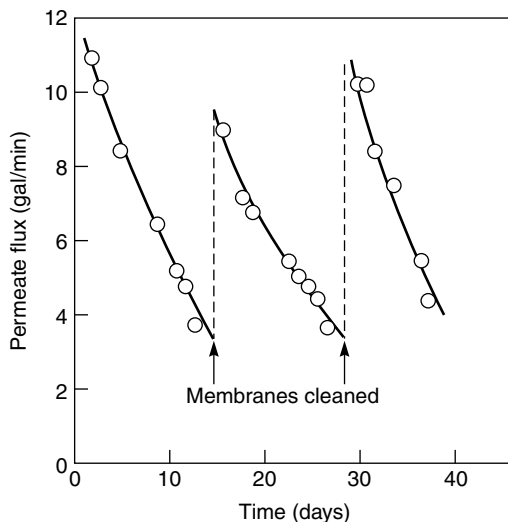
Figure 6.5 Ultrafiltration flux as a function of time of an electrocoat paint latex solution. Because of fouling, the flux declines over a period of days. Periodic cleaning is required to maintain high fluxes [14]. Reprinted from R. Walker, Recent Developments in Ultrafiltration of Electrocoat Paint, Electrocoat 82 , 16 (1982) with permission from Gardner Publications, Inc., Cincinnati, OH
