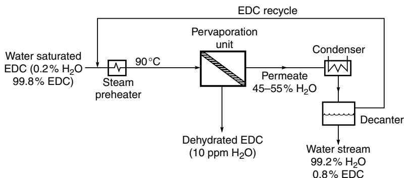
Figure 9.13 Other solvent dehydration processes under investigation
