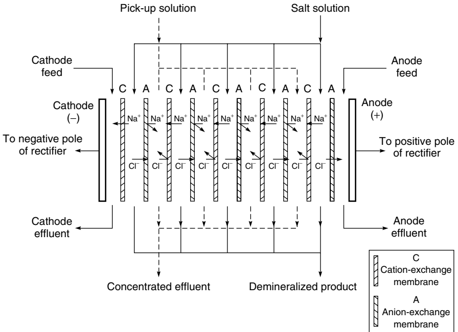
Figure 10.2 Schematic diagram of a plate-and-frame electrodiolysis stack. Alternating cation- and anion-permeable membranes are arranged in a stack of up to 100 cell pairs
