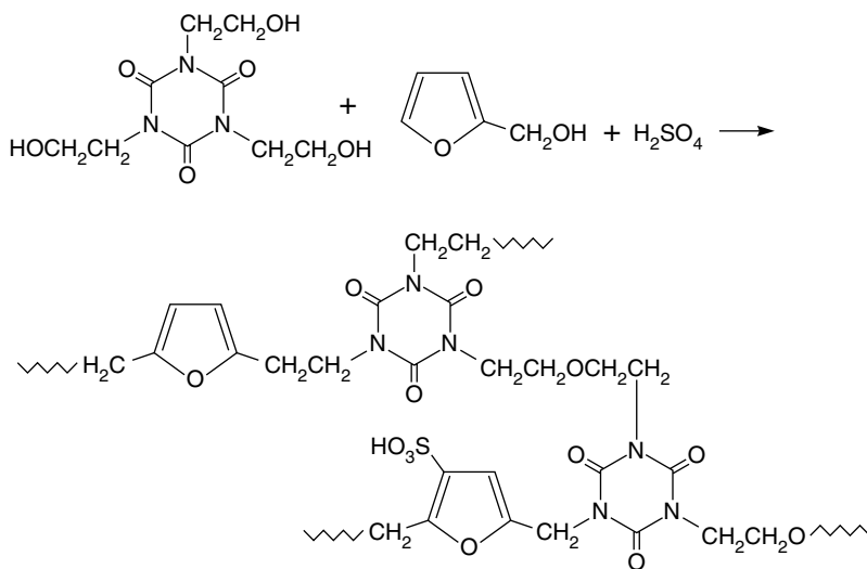
Figure 5.11 Reaction sequence for Toray's PEC-1000 membrane
