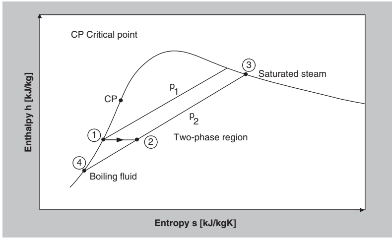
Figure 2.18 Enthalpy-entropy (h-s) diagram for flash evaporation process.
