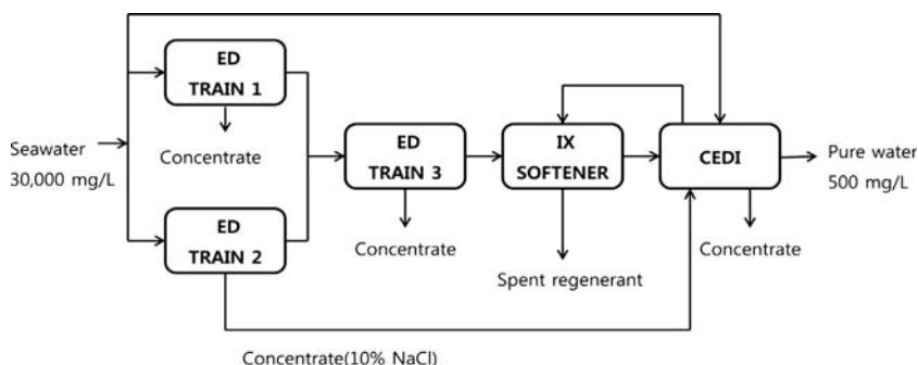
Figure 6.10 Low energy ED system and process for seawater desalination [56].
