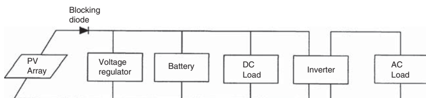
Figure 13.18 Schematic of a stand-alone photovoltaic system
