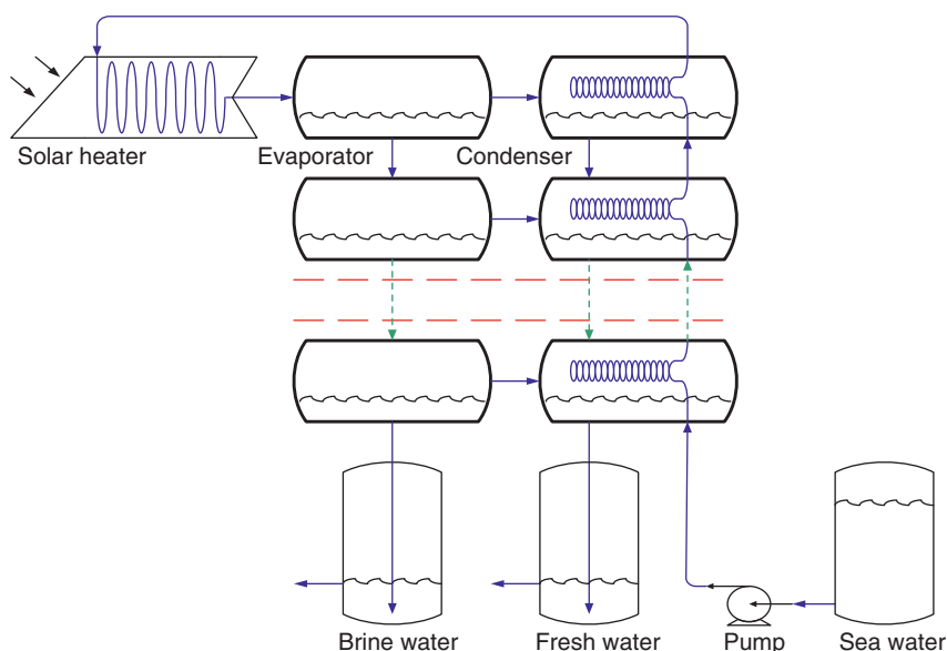
Figure 13.13 Multi-stage solar flash desalination system
