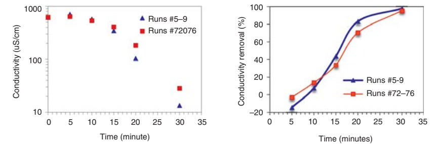
Figure 12.3 Variation of conductivity of the electrolyte during experimental Runs #5-9 and #72-76.
