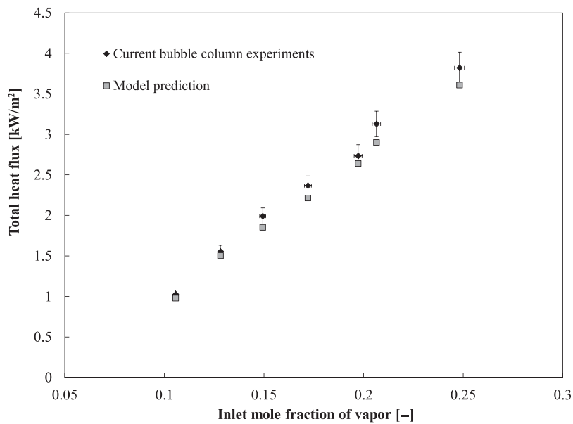
Figure 9.23 Effect of inlet mole fraction of the vapor on the total heat flux in the bubble column measured and evaluated at Vg = 3.8 \text{ cm/s} ; D_b = 4 \text{ mm} ; H = 254 \text{ mm} [66].
