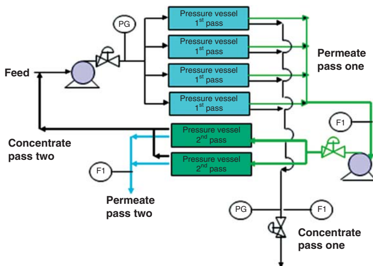
Figure 3.17 Schematic configuration of two pass RO unit.
