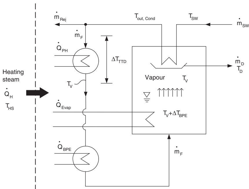
Figure 2.12 Flow scheme of a single-stage evaporation process with energy recovery.
