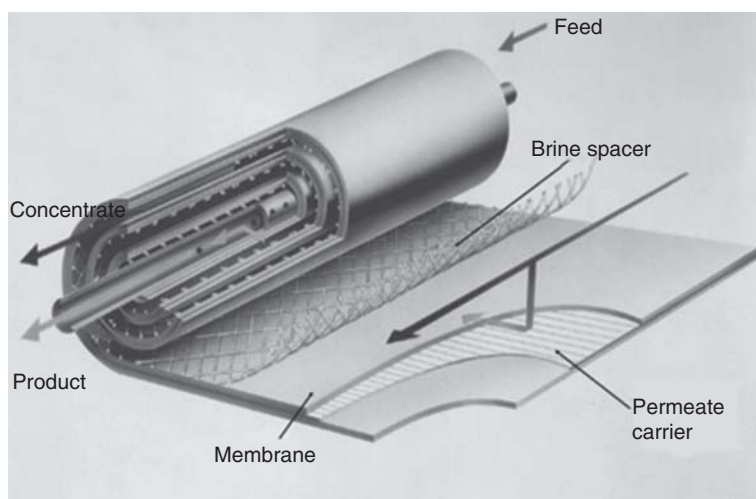
Figure 3.9 Configuration of spiral wound membrane element.
