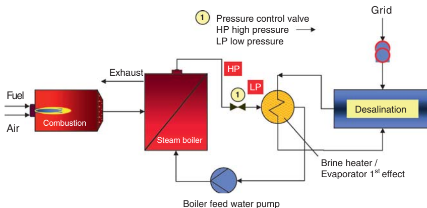
Figure 2.40 Flow sheet of a single purpose plant (steam boiler + desalination).
