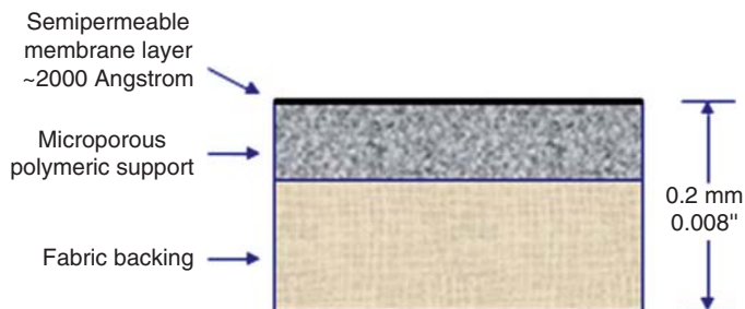
Figure 3.5 Cross section configuration of flat sheet RO membrane.
