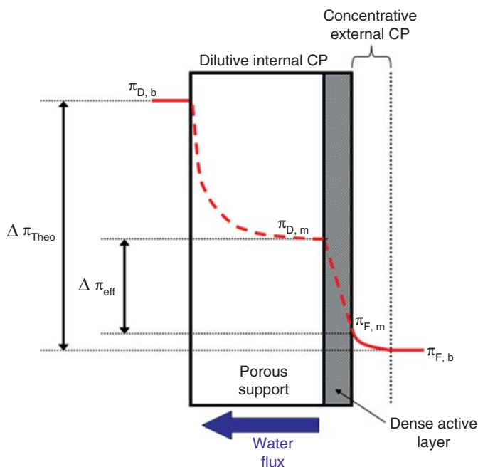
Figure 5.4 – Illustration of concentration polarization phenomenon near the active (selective) layer of the membrane. \pi refers to the osmotic pressure of the solution. \Delta\pi is indicative of the osmotic driving force across the membrane while the subscripts “Theo” and “eff” refer to the theoretical and effective driving force, respectively. Subscripts D, F, m, and b refer to the “draw”, “feed”, “selective layer interface”, and “bulk” osmotic pressures, respectively
