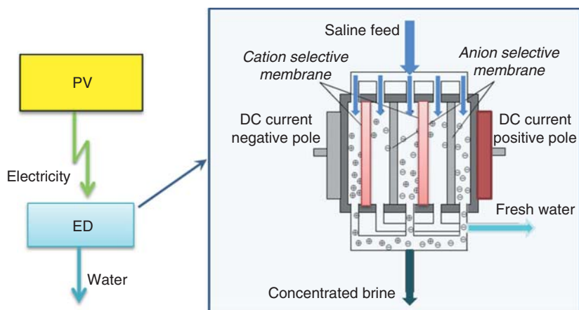
Figure 13.10 PV assisted electro-dialysis
