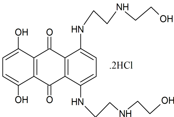
Figure 8. Molecular structure of Mitoxantrone.
