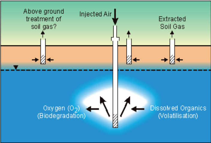
Figure 3. Air Sparging [31]
