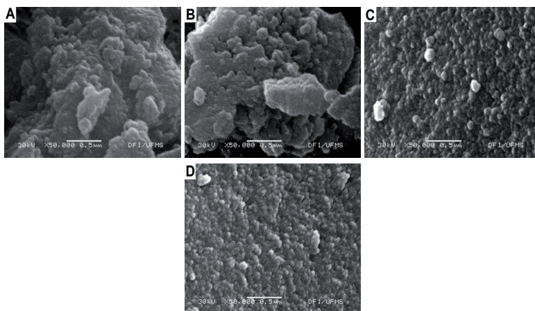
Figure 11. Scanning electron micrographs of: (A) \text{TiO}_2 SG 0.5% Ag; (B) \text{TiO}_2 SG 1.0% Ag; (C) \text{TiO}_2 SG 2.0% Ag; (D) \text{TiO}_2 SG 4.0% Ag.
