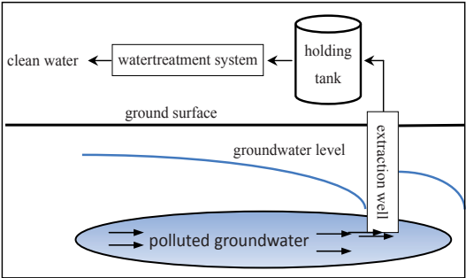
Figure 2. Pump and Treat Technology [29]
