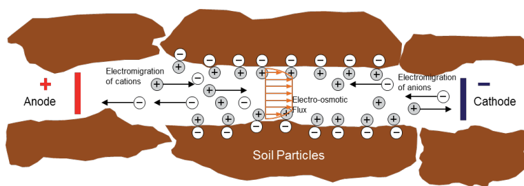
Figure 2. Transport mechanisms in electrokinetic remediation
