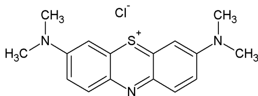
Figure 15. Molecular structure of Methylene Blue.
