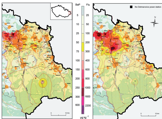
Figure 3. The load of the North Moravian Region by benzo(a)pyrene and fluoranthene ( \mu\text{g/kg} )
