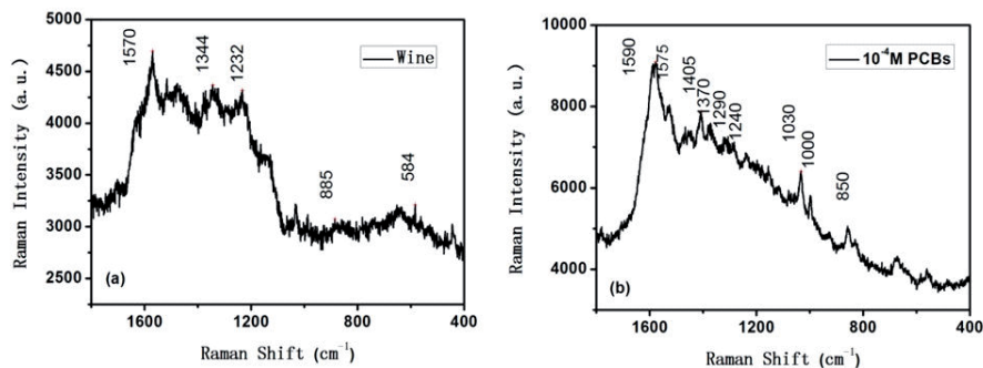
Figure 14. SERS spectra of white spirit without and with PCBs.
