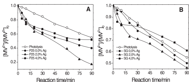
Figure 12. Results of MV^{2+} ( 0.2 \text{ mmol L}^{-1} ) degradation by heterogeneous photocatalysis ( 0.5 \text{ g} of photocatalyst) with (A) TiO_2 P25 and (B) TiO_2 SG.
