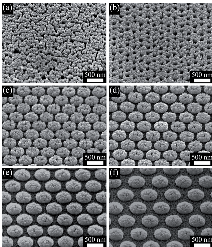
Figure 8. Oblique-view SEM images of vertically aligned Ag nanorods deposited on (a) unpatterned silicon; and on hexagonal lattices of silicon patterns that are separated by (b) 0 nm (closely-packed); (c) 50 nm; (d) 100 nm; (e) 200 nm; and (f) 300 nm, respectively.
