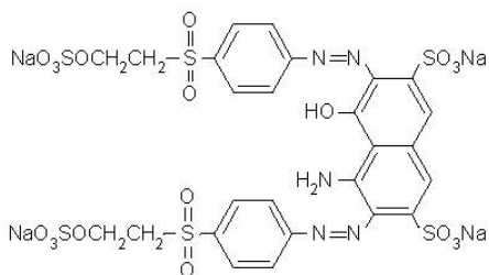
Figure 3. Chemical structure of reactive black 5
