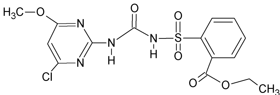
Figure 6. Molecular structure of Chlorimurom-ethyl (CE).
