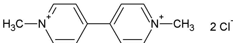
Figure 10. Molecular structure of Methyl Viologen.
