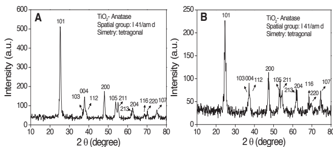
Figure 13. X-ray diffractograms of \text{TiO}_2 synthesized by the molten salt method: (A) in \text{NaNO}_3 and (B) in \text{KNO}_3 .
