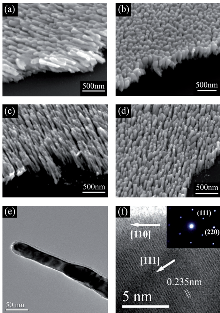
Figure 1. Growth morphology of thin Ag films by GLAD at various conditions. (a) at 120^{\circ}\text{C} without substrate rotation; (b) at 120^{\circ}\text{C} and substrate rotation at 0.2 rpm; (c) at -40^{\circ}\text{C} without substrate rotation; and (d) at -40^{\circ}\text{C} and substrate rotation at 0.2 rpm. (e) and (f) shows respectively a bright-field TEM and a HRTEM image of the nanorods shown by Fig 1(c); inset of (f) is the corresponding SAD pattern.
