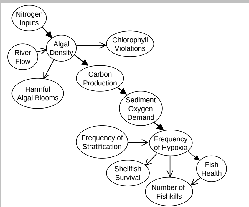
FIGURE 1 Probability network model for the Neuse Estuary TMDL development.
