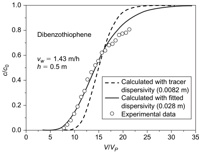
Figure 9.5 Comparison of the conventional and the extended LEM (dibenzothiophene/sandy aquifer material). Experimental data from Schreiber (2002).
