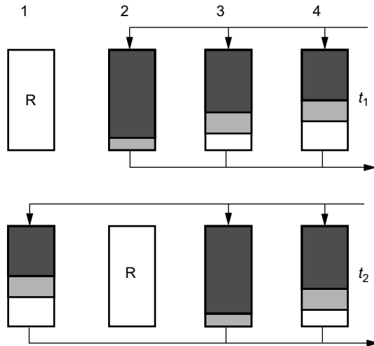
Figure 6.18 Fixed-bed adsorbers in parallel connection. Legend: R, adsorber out of operation for adsorbent regeneration; dark gray, adsorbent loaded to equilibrium; light gray, MTZ; white, adsorbent free of adsorbate.
