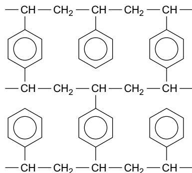
Figure 2.2 Structure of a styrene-divinylbenzene copolymer.
