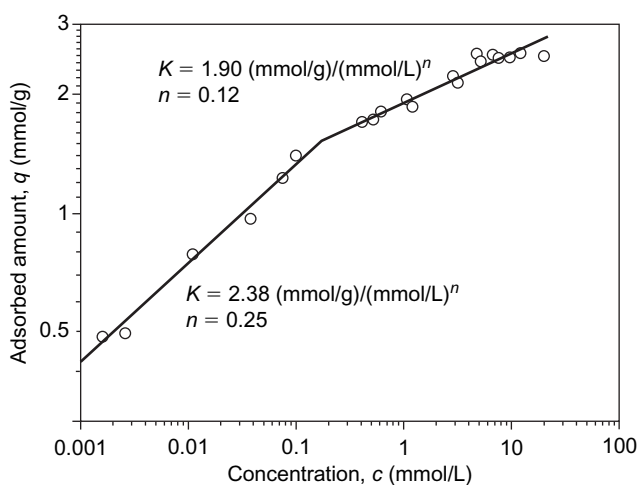
Figure 3.8 Description of an isotherm over a broad concentration range by using different sets of Freundlich parameters (4-chlorophenol – activated carbon DO4).
