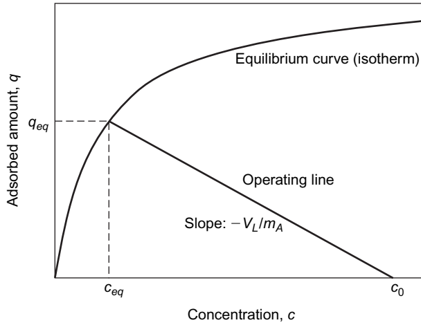
Figure 3.17 Operating line for single-stage adsorption.
