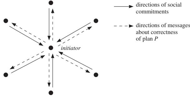
Figure 4.1 Team structure of the star topology illustrating the messages and social commitments. The initiator first sends individual messages ‘ constitute ( \varphi, P )’ to all team members and after each a \in G pronounces its social commitment \text{COMM}(a, \text{initiator}, \alpha) , the initiator sends each team member individually the message ‘ \bigwedge_{\alpha \in P} \bigvee_{a \in G \setminus \{\text{initiator}\}} \text{COMM}(a, \text{initiator}, \alpha) ’.
