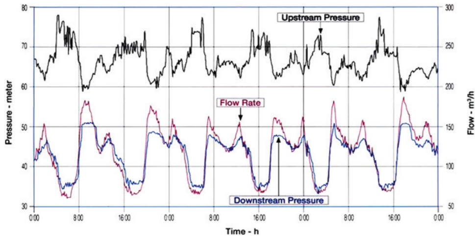
Figure 3.9 Flow modulated pressure control.
