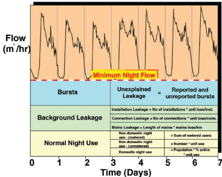
Figure 6.2 Interpretation of the minimum night flow.
