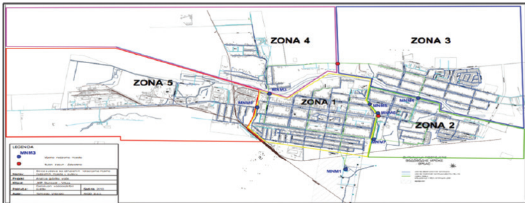
Figure 9.3.3 Vrbas water distribution network with future DMA zones (Source: Water Loss Audit report, Kovac, 2010).
