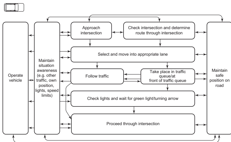
FIGURE 7.2 Driver intersection task network.
