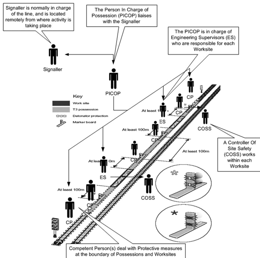
FIGURE 6.2 Overall diagram of the various track possession scenarios.
