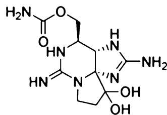
Fig. 13.1 Saxitoxin
