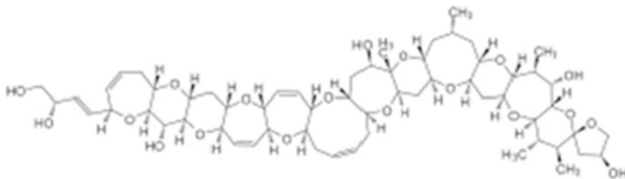
Fig. 11.3 Structure of ciguatera toxin
