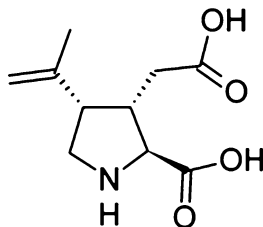
Fig. 11.4 Structure of kainic acid
