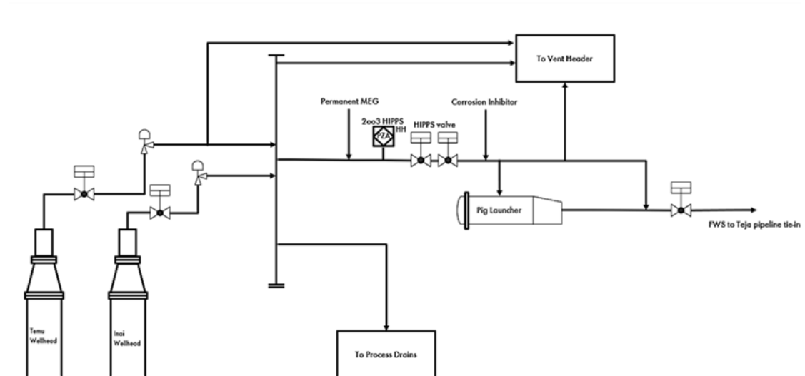
Simplified Process Flow Diagram Illustration Teja FWS to Pepulut, TuNai to Teja, and Pepulut FWS to F23
