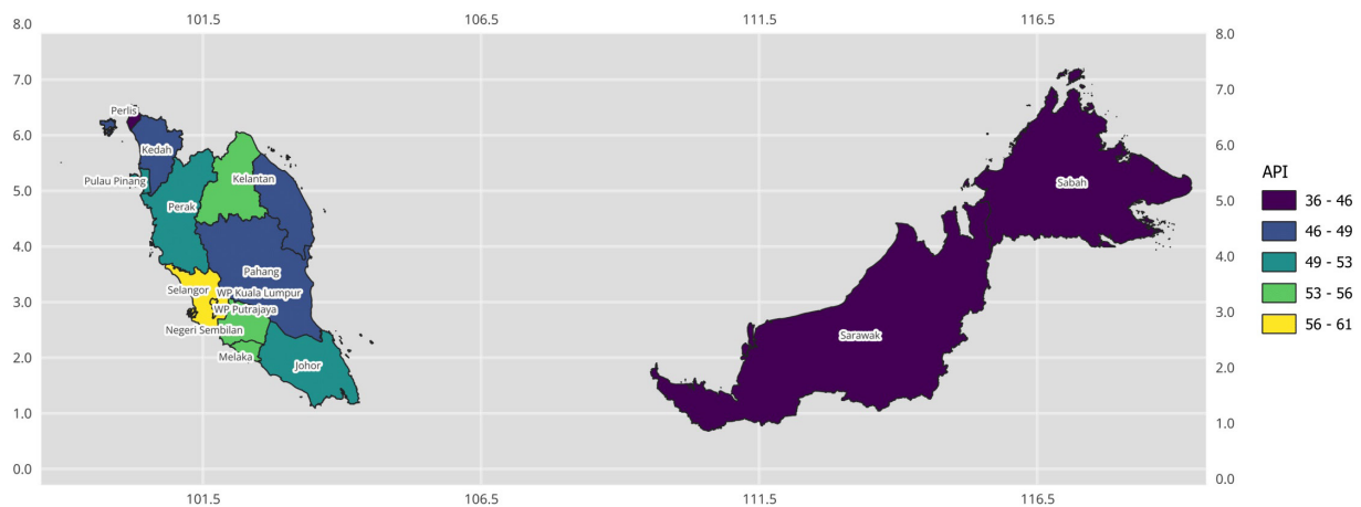
Rajah 1.3: Purata Indeks Pencemaran Udara (IPU) di Malaysia Figure 1.3: The Average Air Pollutant Index (API) in Malaysia
