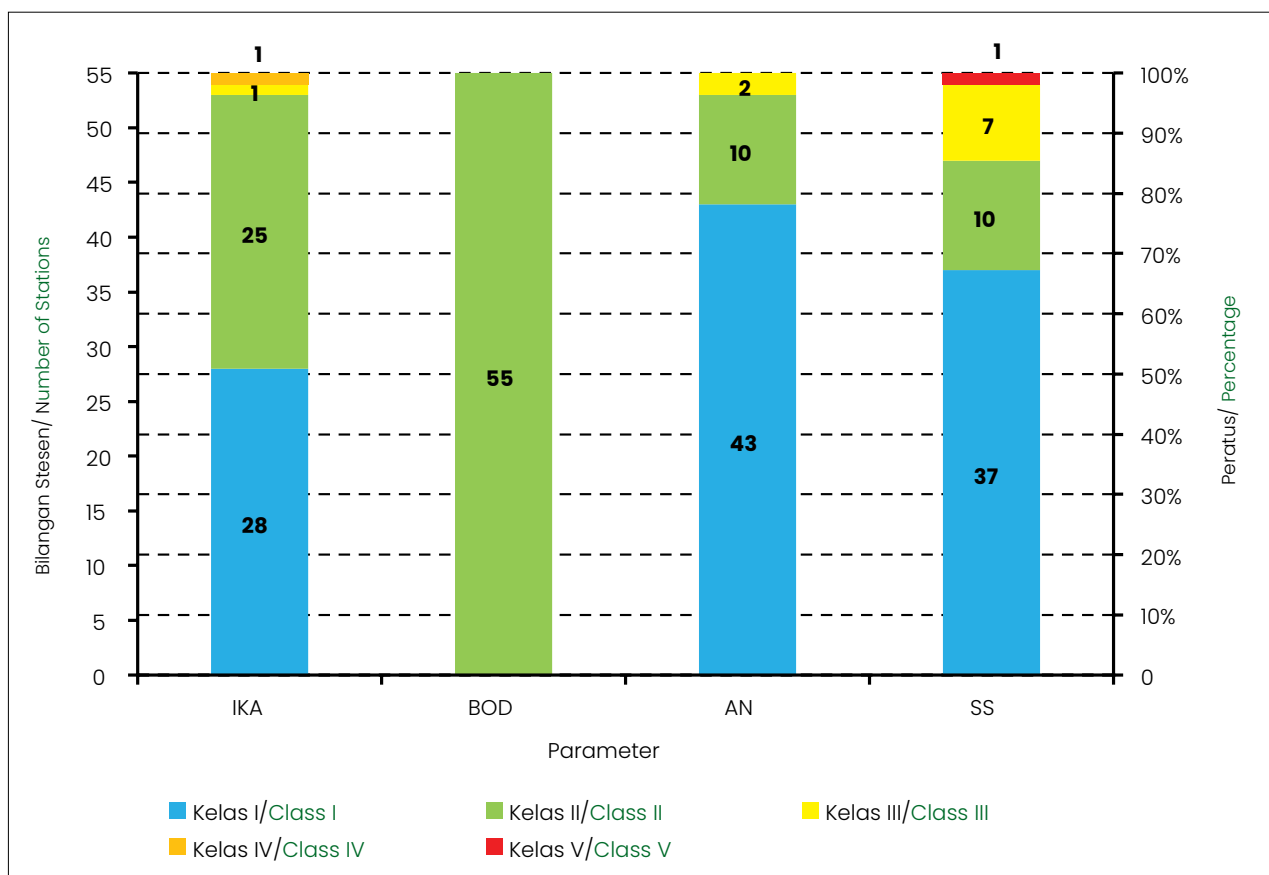
Rajah 2.9 : Kualiti Air Sungai di Stesen Hulu Muka Sauk, 2024 Figure 2.9 : River Water Quality at Upstream Water Intake Stations, 2024
